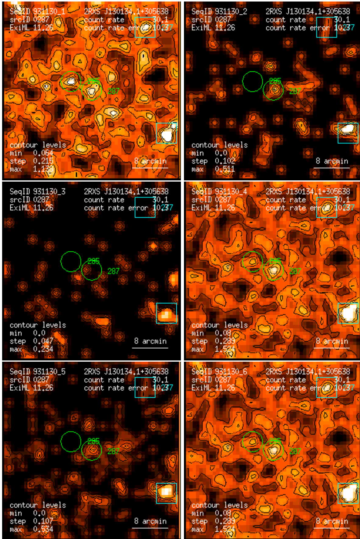
Figure 287: RASS 931130: detection 0287: band rate images, Gaussian filter: (1) PSPC channels 11 – 41, (2) 52 – 90, (3) 91 – 201, (4) 11 – 235, (5) 52 – 201, (6) 11 – 201. Broad band rates in counts/ks. Band rate contour levels in counts/ks/arcmin 2 .
