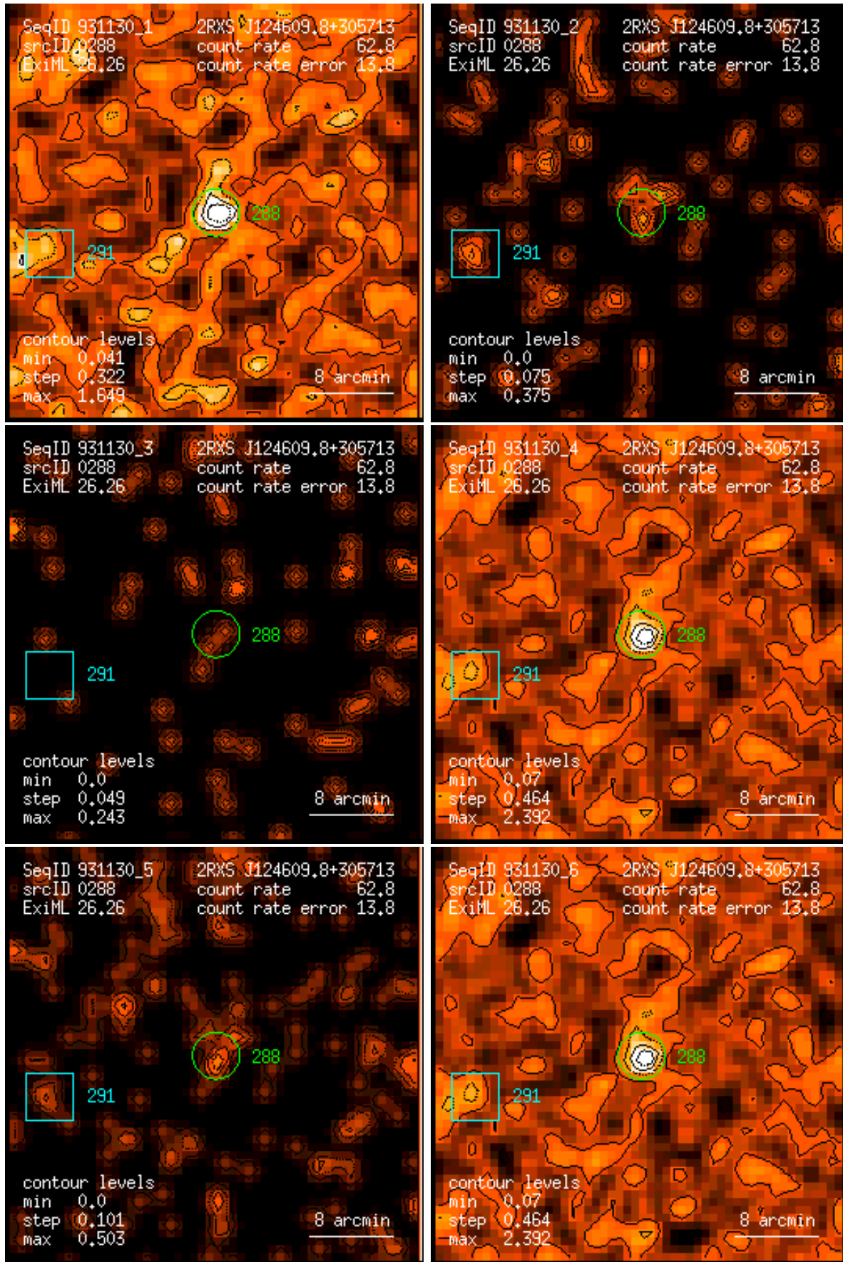
Figure 288: RASS 931130: detection 0288: band rate images, Gaussian filter: (1) PSPC channels 11 – 41, (2) 52 – 90, (3) 91 – 201, (4) 11 – 235, (5) 52 – 201, (6) 11 – 201. Broad band rates in counts/ks. Band rate contour levels in counts/ks/arcmin 2 .
