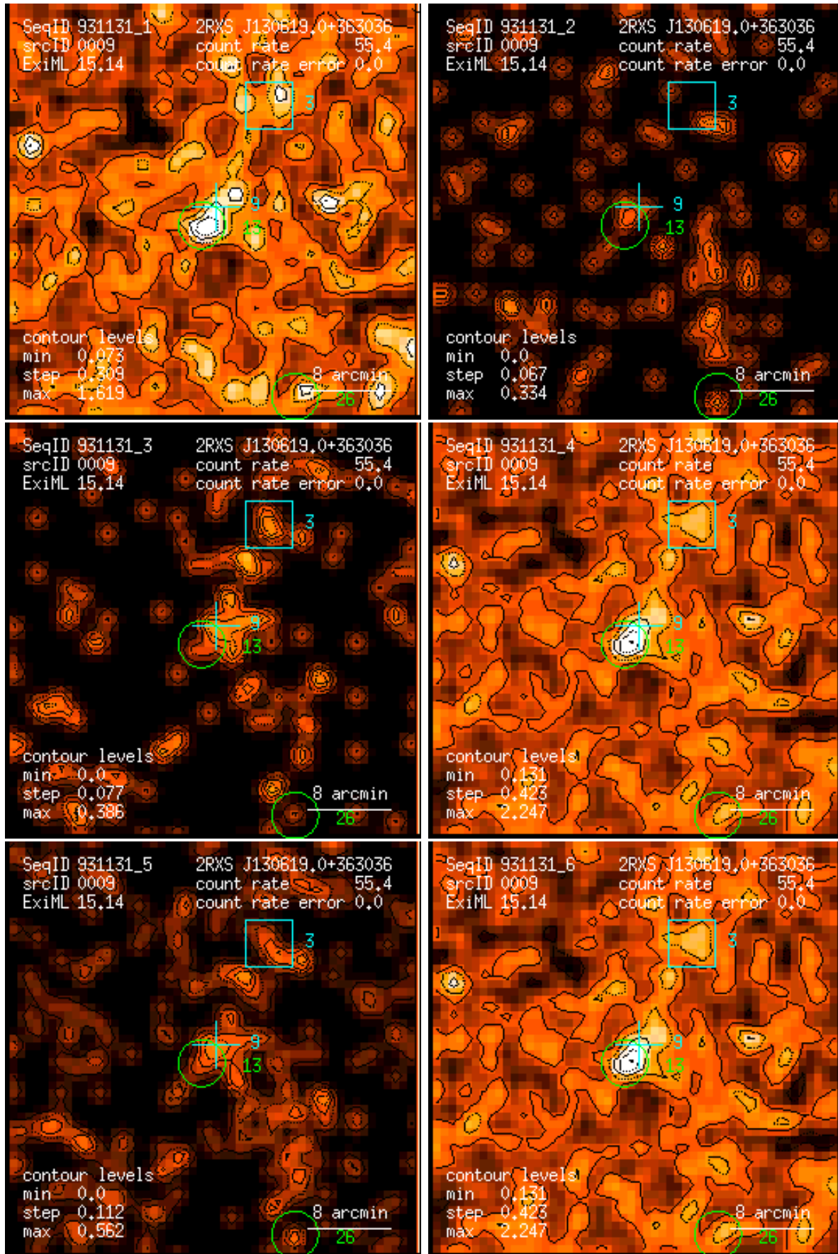
Figure 9: RASS 931131: detection 0009: band rate images, Gaussian filter: (1) PSPC channels 11 – 41, (2) 52 – 90, (3) 91 – 201, (4) 11 – 235, (5) 52 – 201, (6) 11 – 201. Broad band rates in counts/ks. Band rate contour levels in counts/ks/arcmin 2 .
