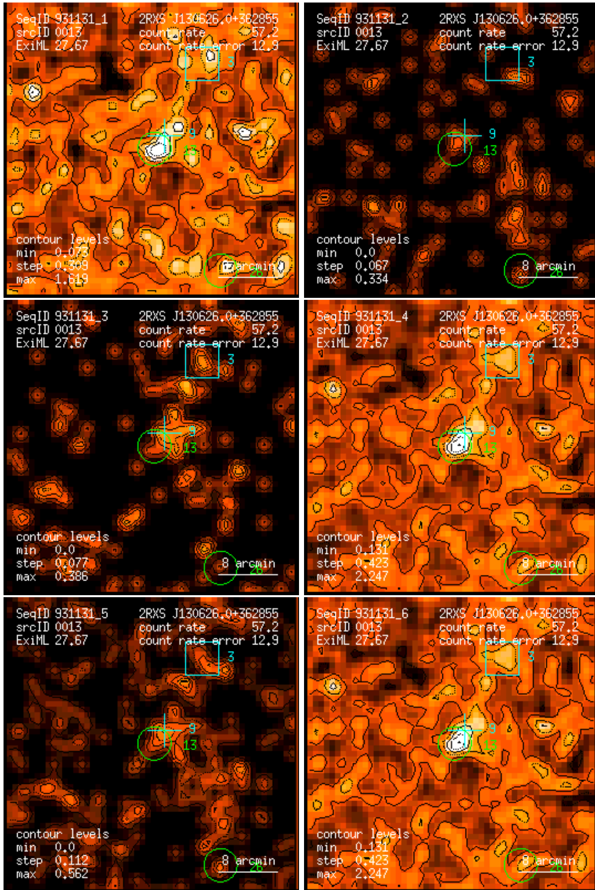
Figure 13: RASS 931131: detection 0013: band rate images, Gaussian filter: (1) PSPC channels 11 – 41, (2) 52 – 90, (3) 91 – 201, (4) 11 – 235, (5) 52 – 201, (6) 11 – 201. Broad band rates in counts/ks. Band rate contour levels in counts/ks/arcmin 2 .
