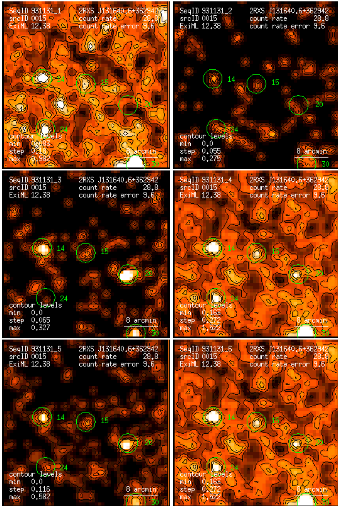
Figure 15: RASS 931131: detection 0015: band rate images, Gaussian filter: (1) PSPC channels 11 – 41, (2) 52 – 90, (3) 91 – 201, (4) 11 – 235, (5) 52 – 201, (6) 11 – 201. Broad band rates in counts/ks. Band rate contour levels in counts/ks/arcmin 2 .
