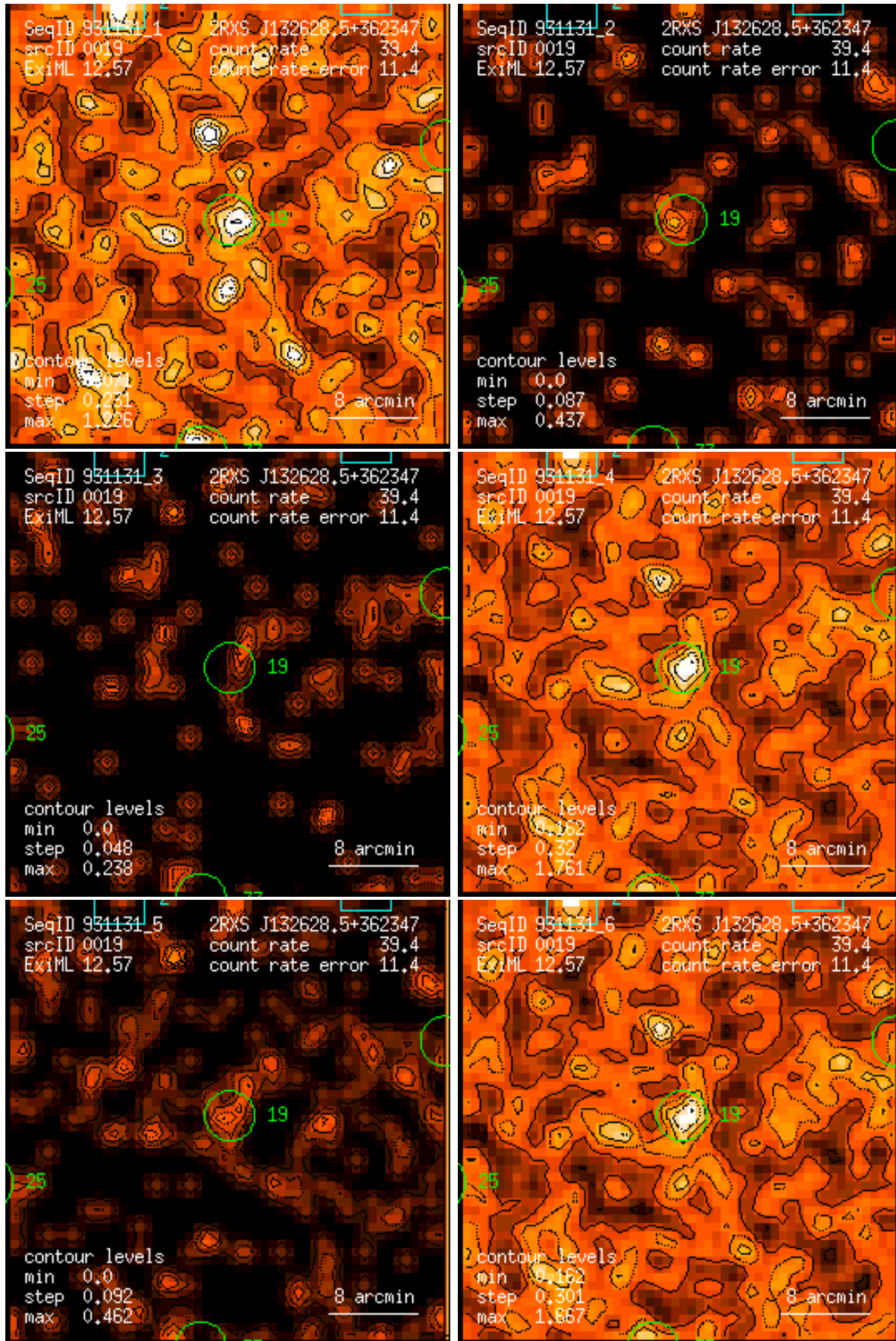
Figure 19: RASS 931131: detection 0019: band rate images, Gaussian filter: (1) PSPC channels 11 – 41, (2) 52 – 90, (3) 91 – 201, (4) 11 – 235, (5) 52 – 201, (6) 11 – 201. Broad band rates in counts/ks. Band rate contour levels in counts/ks/arcmin 2 .
