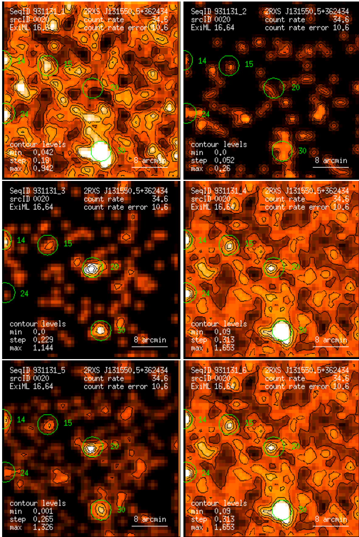
Figure 20: RASS 931131: detection 0020: band rate images, Gaussian filter: (1) PSPC channels 11 – 41, (2) 52 – 90, (3) 91 – 201, (4) 11 – 235, (5) 52 – 201, (6) 11 – 201. Broad band rates in counts/ks. Band rate contour levels in counts/ks/arcmin 2 .
