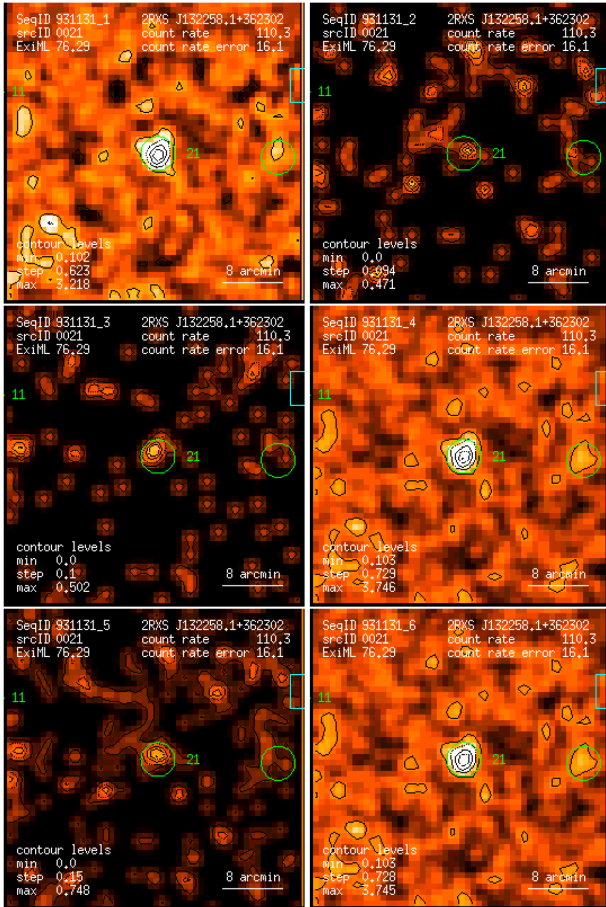
Figure 21: RASS 931131: detection 0021: band rate images, Gaussian filter: (1) PSPC channels 11 – 41, (2) 52 – 90, (3) 91 – 201, (4) 11 – 235, (5) 52 – 201, (6) 11 – 201. Broad band rates in counts/ks. Band rate contour levels in counts/ks/arcmin 2 .
