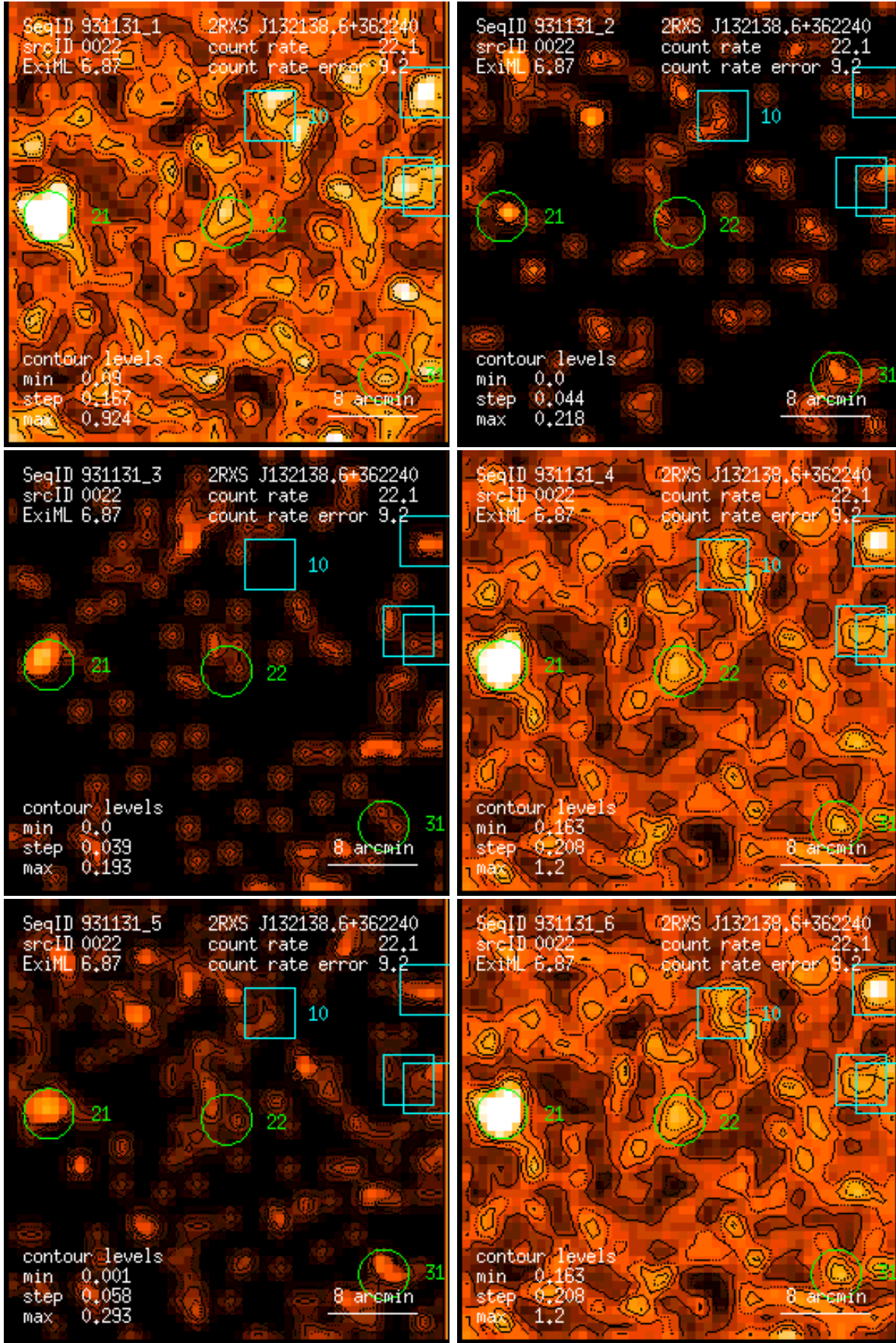
Figure 22: RASS 931131: detection 0022: band rate images, Gaussian filter: (1) PSPC channels 11 – 41, (2) 52 – 90, (3) 91 – 201, (4) 11 – 235, (5) 52 – 201, (6) 11 – 201. Broad band rates in counts/ks. Band rate contour levels in counts/ks/arcmin 2 .
