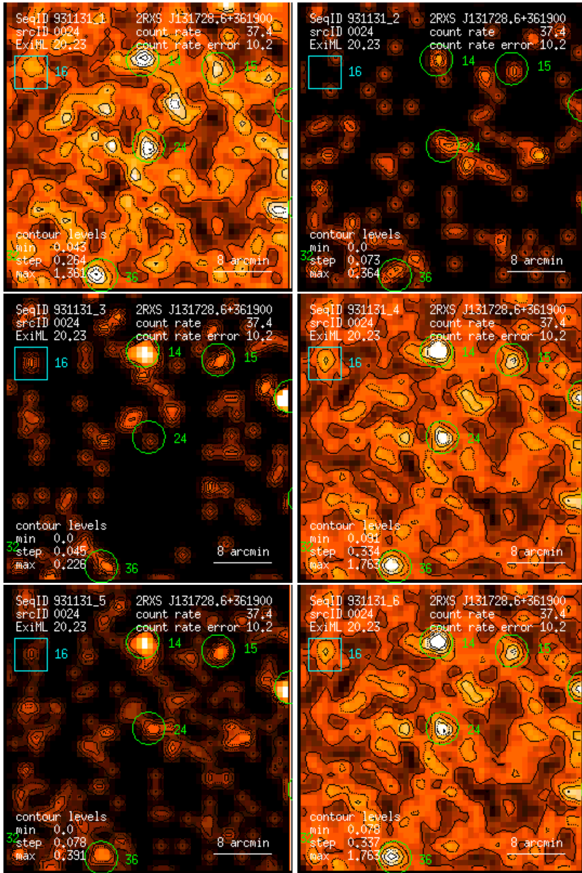
Figure 24: RASS 931131: detection 0024: band rate images, Gaussian filter: (1) PSPC channels 11 – 41, (2) 52 – 90, (3) 91 – 201, (4) 11 – 235, (5) 52 – 201, (6) 11 – 201. Broad band rates in counts/ks. Band rate contour levels in counts/ks/arcmin 2 .
