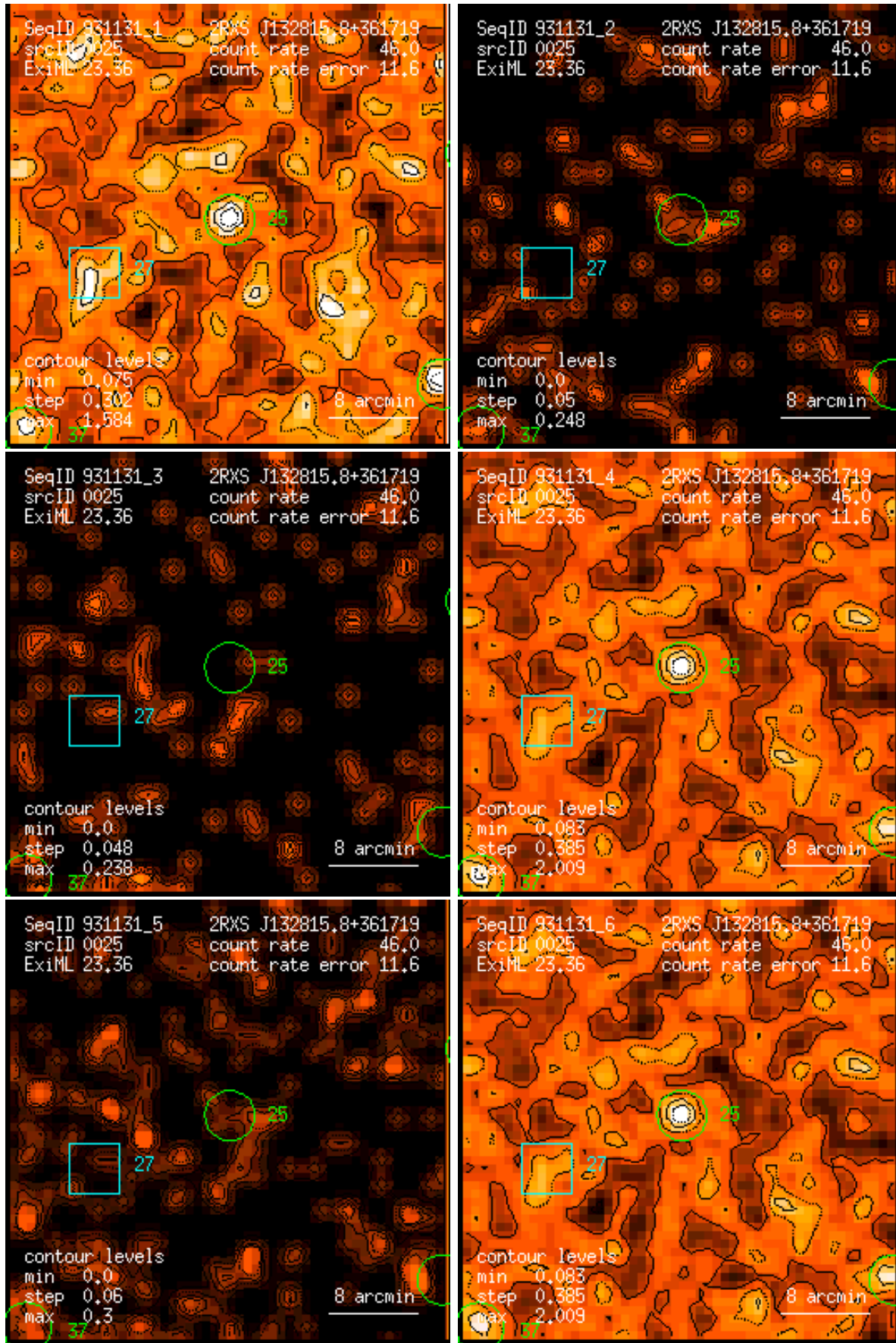
Figure 25: RASS 931131: detection 0025: band rate images, Gaussian filter: (1) PSPC channels 11 – 41, (2) 52 – 90, (3) 91 – 201, (4) 11 – 235, (5) 52 – 201, (6) 11 – 201. Broad band rates in counts/ks. Band rate contour levels in counts/ks/arcmin 2 .
