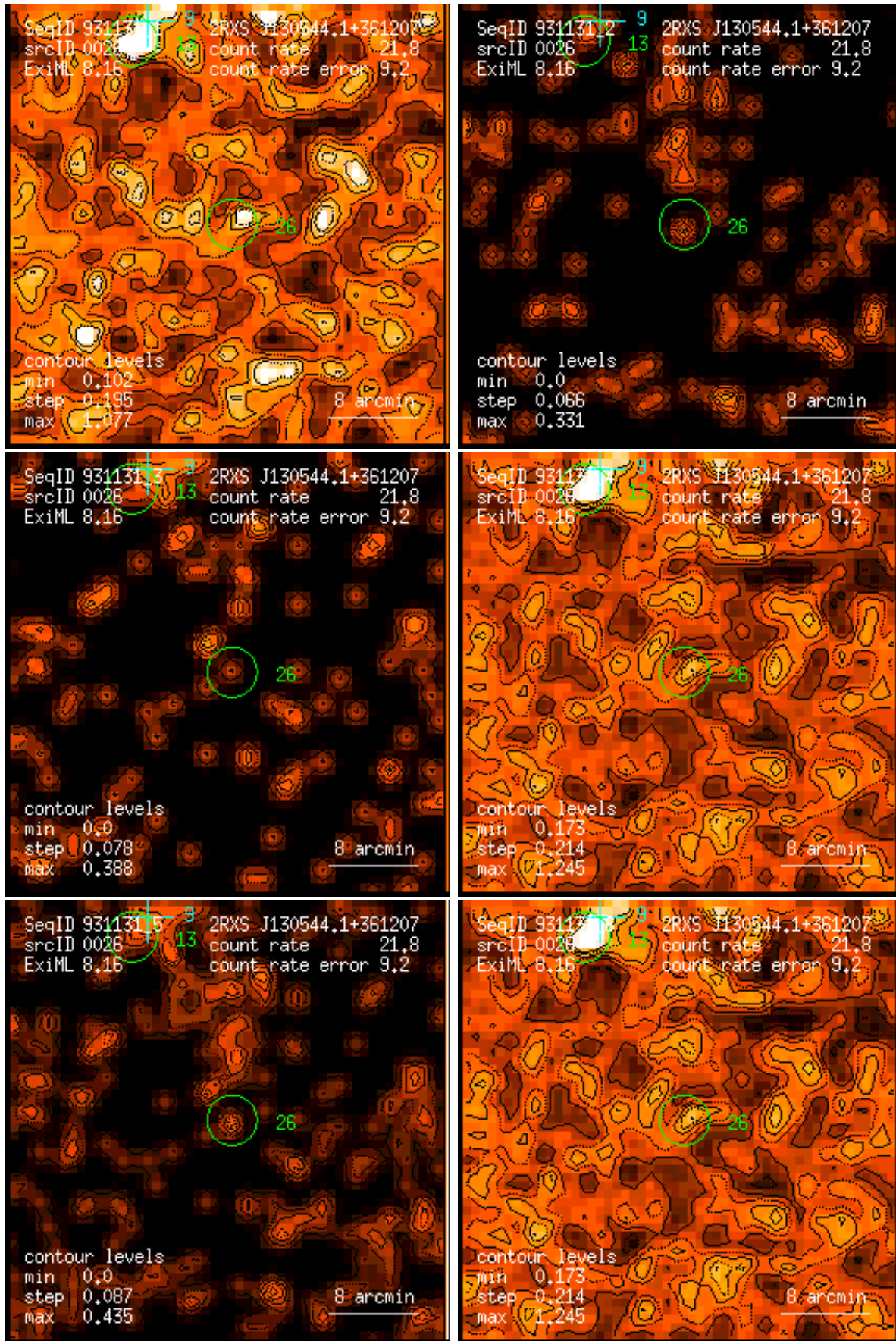
Figure 26: RASS 931131: detection 0026: band rate images, Gaussian filter: (1) PSPC channels 11 – 41, (2) 52 – 90, (3) 91 – 201, (4) 11 – 235, (5) 52 – 201, (6) 11 – 201. Broad band rates in counts/ks. Band rate contour levels in counts/ks/arcmin 2 .
