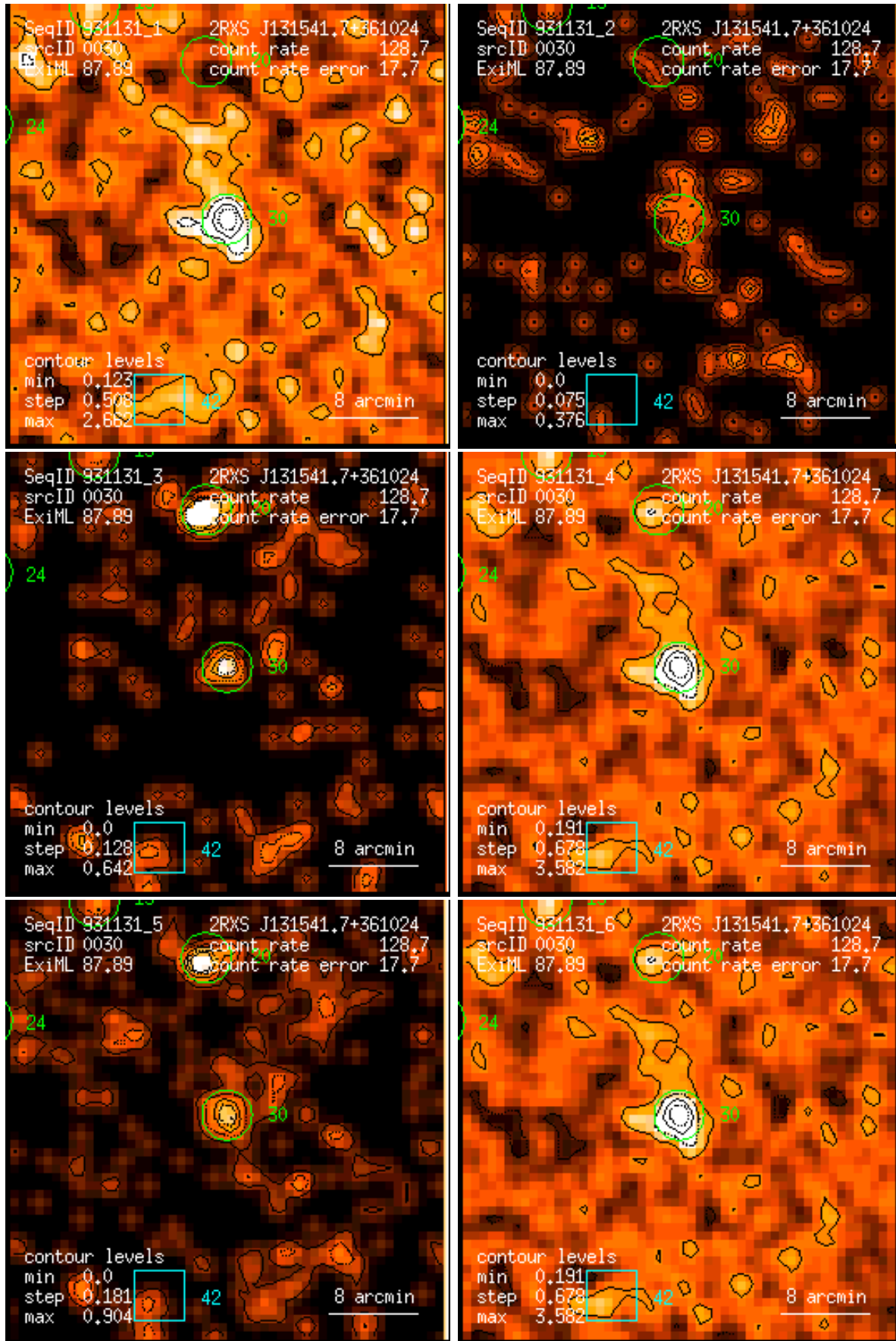
Figure 30: RASS 931131: detection 0030: band rate images, Gaussian filter: (1) PSPC channels 11 – 41, (2) 52 – 90, (3) 91 – 201, (4) 11 – 235, (5) 52 – 201, (6) 11 – 201. Broad band rates in counts/ks. Band rate contour levels in counts/ks/arcmin 2 .
