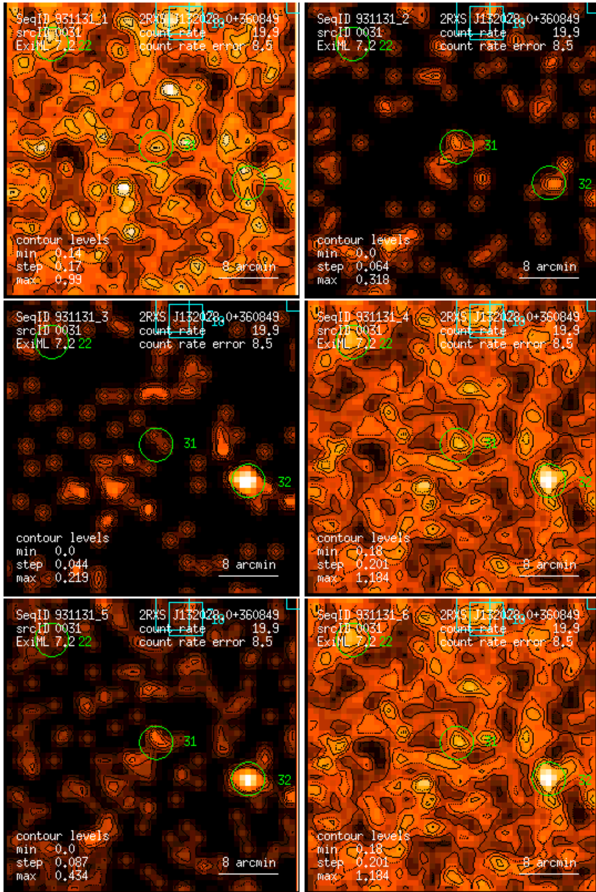
Figure 31: RASS 931131: detection 0031: band rate images, Gaussian filter: (1) PSPC channels 11 – 41, (2) 52 – 90, (3) 91 – 201, (4) 11 – 235, (5) 52 – 201, (6) 11 – 201. Broad band rates in counts/ks. Band rate contour levels in counts/ks/arcmin 2 .
