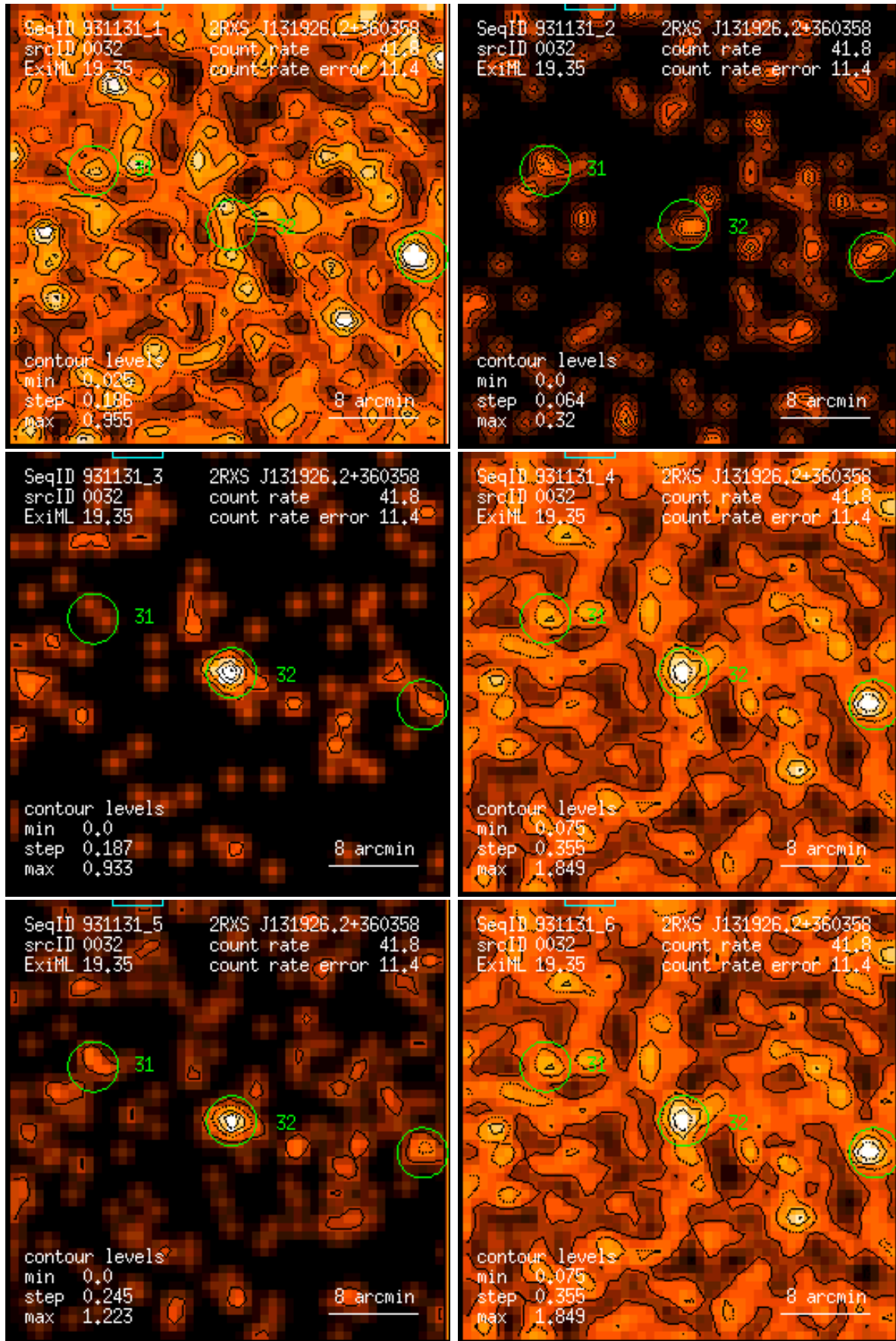
Figure 32: RASS 931131: detection 0032: band rate images, Gaussian filter: (1) PSPC channels 11 – 41, (2) 52 – 90, (3) 91 – 201, (4) 11 – 235, (5) 52 – 201, (6) 11 – 201. Broad band rates in counts/ks. Band rate contour levels in counts/ks/arcmin 2 .
