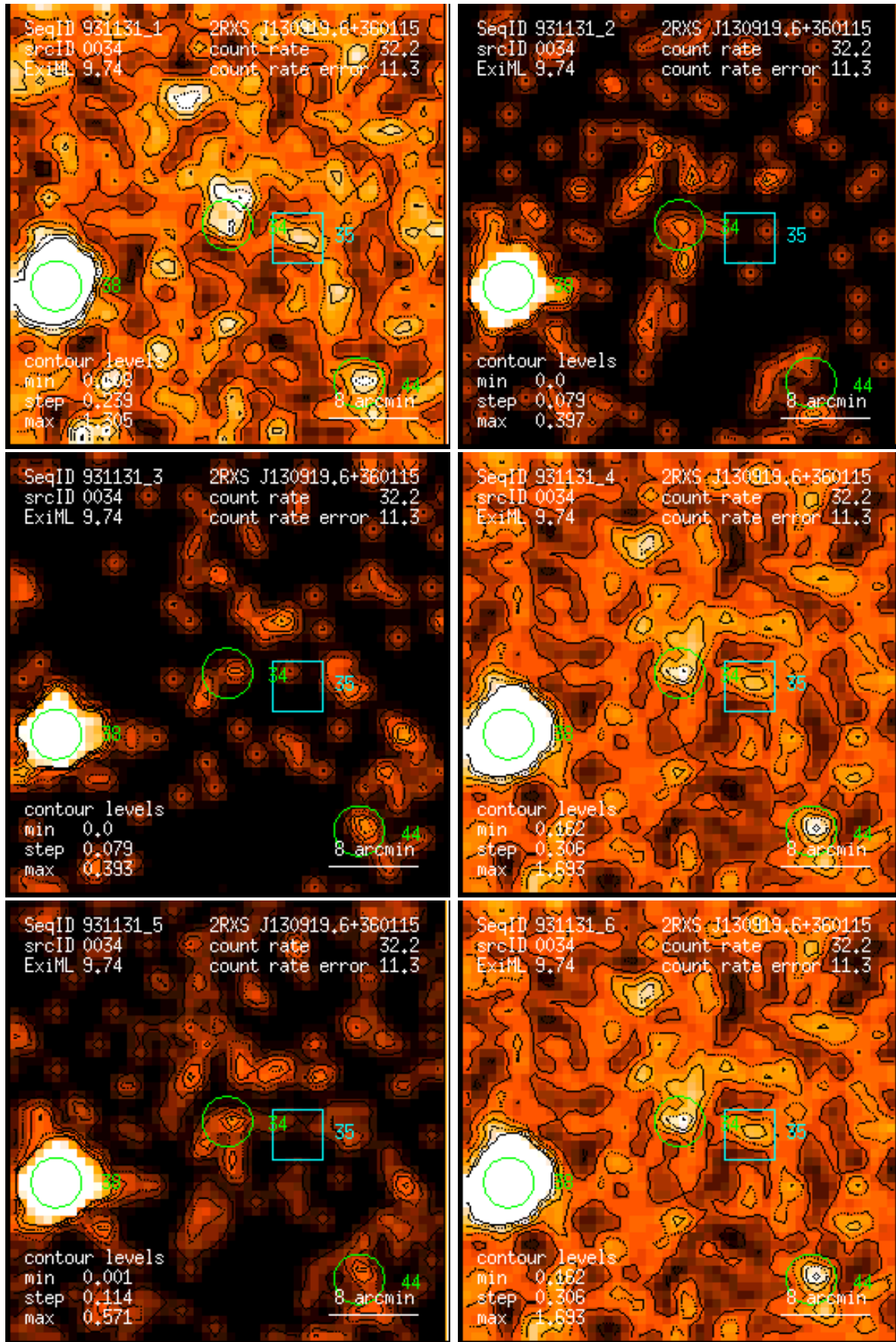
Figure 34: RASS 931131: detection 0034: band rate images, Gaussian filter: (1) PSPC channels 11 – 41, (2) 52 – 90, (3) 91 – 201, (4) 11 – 235, (5) 52 – 201, (6) 11 – 201. Broad band rates in counts/ks. Band rate contour levels in counts/ks/arcmin 2 .
