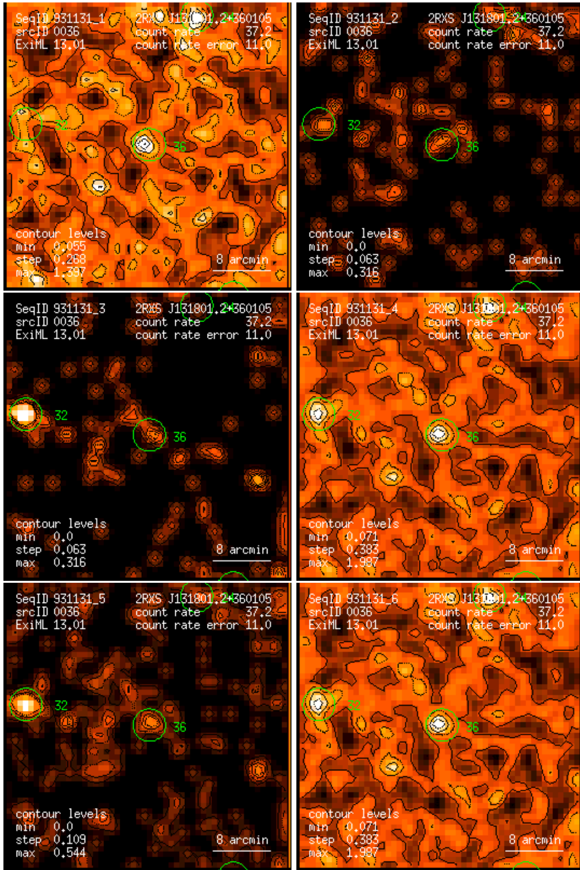
Figure 36: RASS 931131: detection 0036: band rate images, Gaussian filter: (1) PSPC channels 11 – 41, (2) 52 – 90, (3) 91 – 201, (4) 11 – 235, (5) 52 – 201, (6) 11 – 201. Broad band rates in counts/ks. Band rate contour levels in counts/ks/arcmin 2 .
