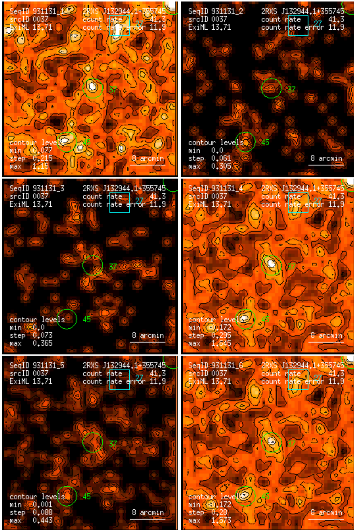
Figure 37: RASS 931131: detection 0037: band rate images, Gaussian filter: (1) PSPC channels 11 – 41, (2) 52 – 90, (3) 91 – 201, (4) 11 – 235, (5) 52 – 201, (6) 11 – 201. Broad band rates in counts/ks. Band rate contour levels in counts/ks/arcmin 2 .
