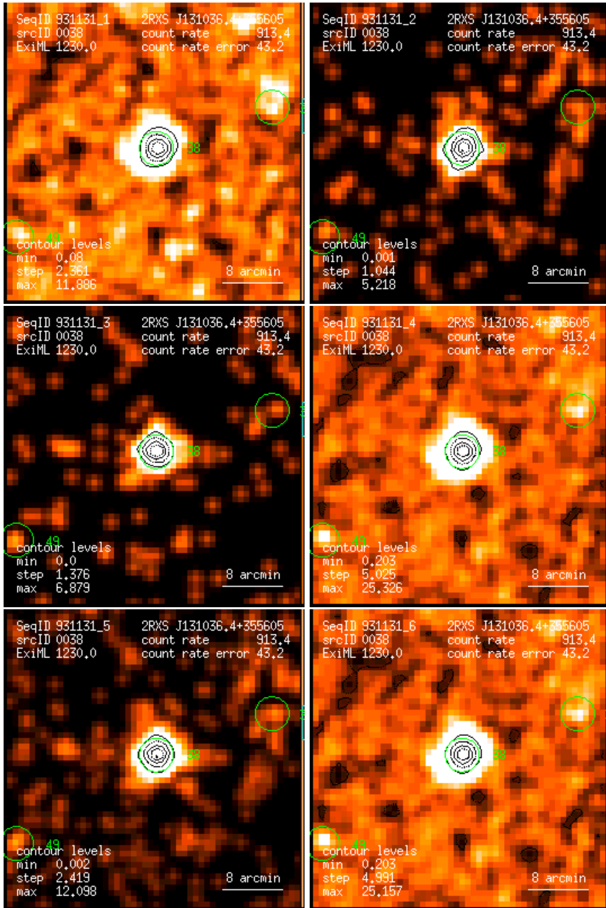
Figure 38: RASS 931131: detection 0038: band rate images, Gaussian filter: (1) PSPC channels 11 – 41, (2) 52 – 90, (3) 91 – 201, (4) 11 – 235, (5) 52 – 201, (6) 11 – 201. Broad band rates in counts/ks. Band rate contour levels in counts/ks/arcmin 2 .
