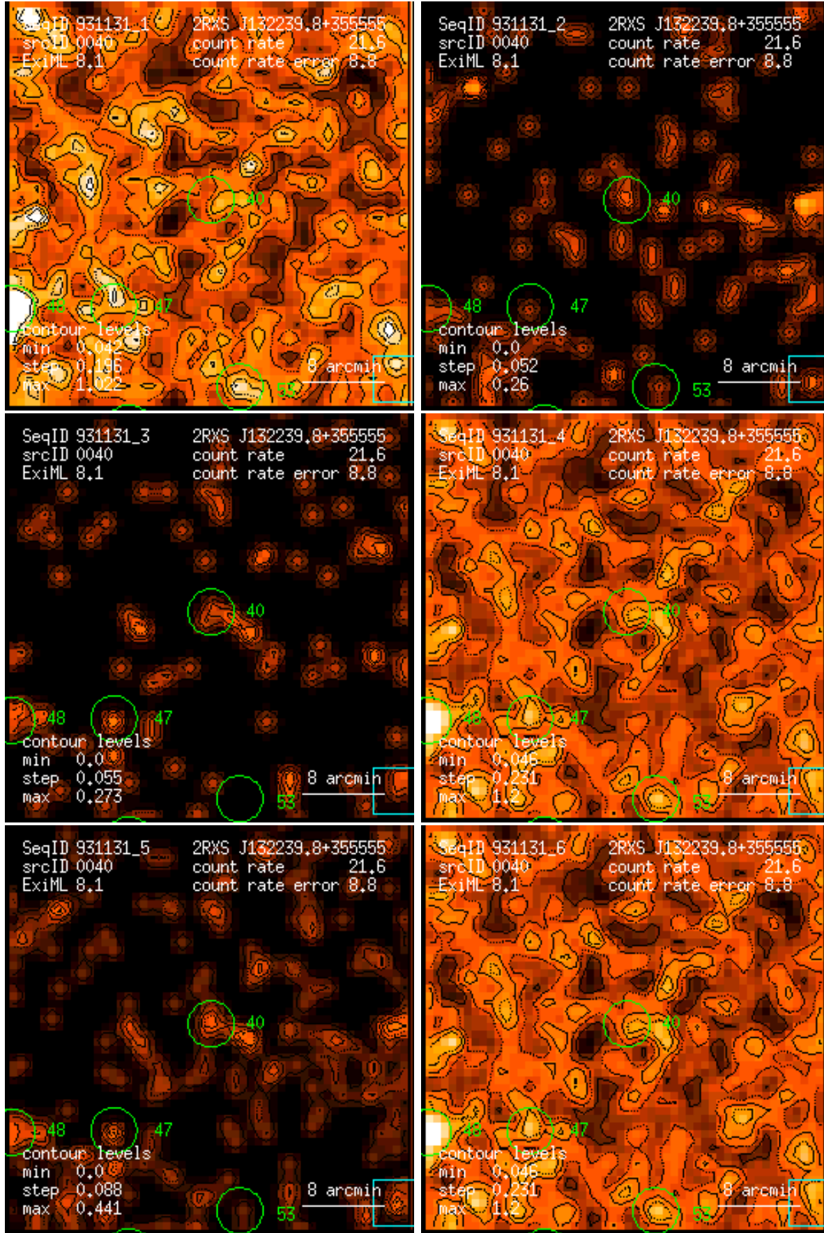
Figure 40: RASS 931131: detection 0040: band rate images, Gaussian filter: (1) PSPC channels 11 – 41, (2) 52 – 90, (3) 91 – 201, (4) 11 – 235, (5) 52 – 201, (6) 11 – 201. Broad band rates in counts/ks. Band rate contour levels in counts/ks/arcmin 2 .
