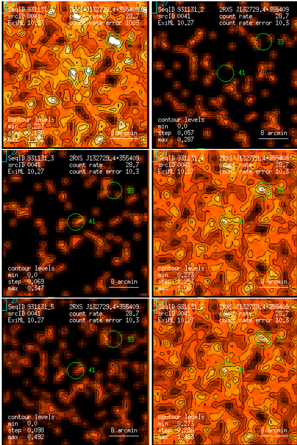
Figure 41: RASS 931131: detection 0041: band rate images, Gaussian filter: (1) PSPC channels 11 – 41, (2) 52 – 90, (3) 91 – 201, (4) 11 – 235, (5) 52 – 201, (6) 11 – 201. Broad band rates in counts/ks. Band rate contour levels in counts/ks/arcmin 2 .
