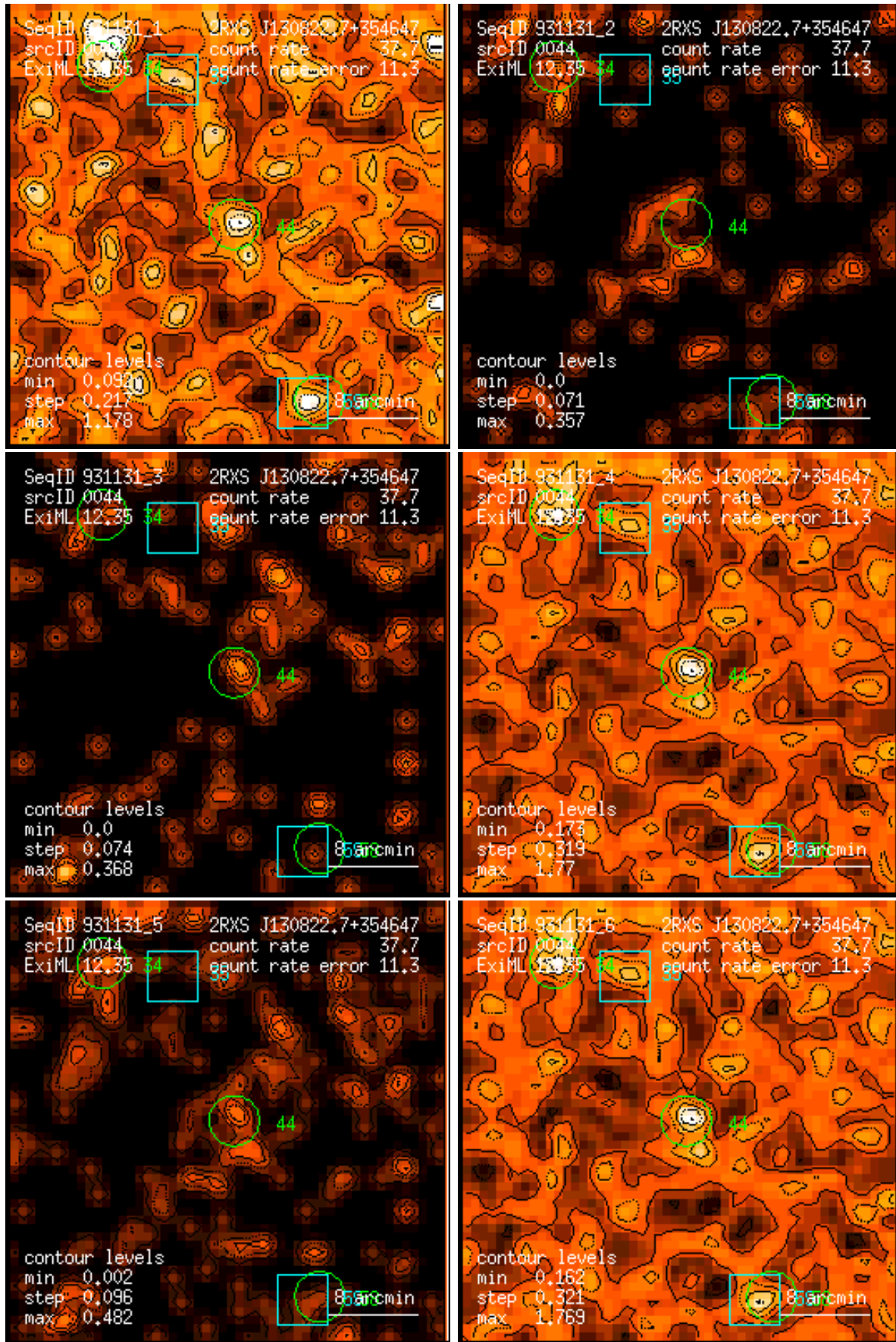
Figure 44: RASS 931131: detection 0044: band rate images, Gaussian filter: (1) PSPC channels 11 – 41, (2) 52 – 90, (3) 91 – 201, (4) 11 – 235, (5) 52 – 201, (6) 11 – 201. Broad band rates in counts/ks. Band rate contour levels in counts/ks/arcmin 2 .
