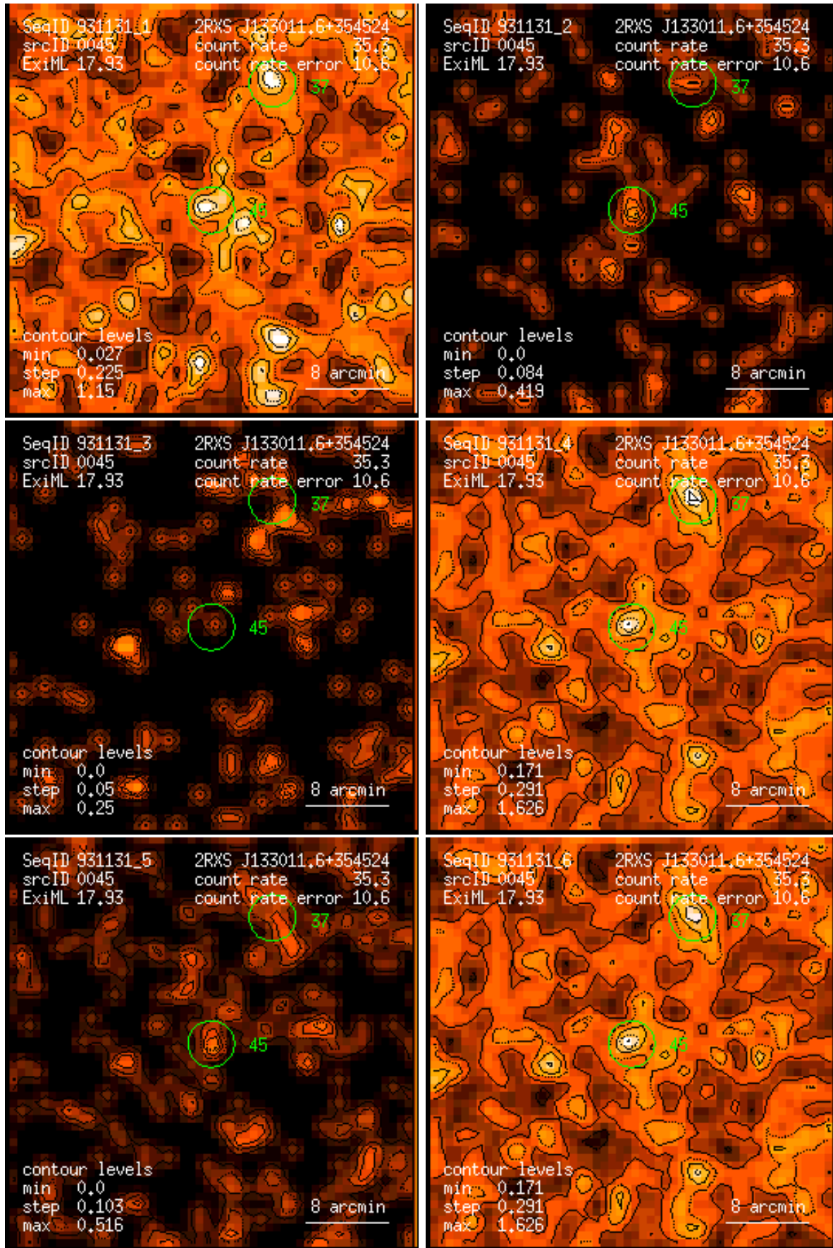
Figure 45: RASS 931131: detection 0045: band rate images, Gaussian filter: (1) PSPC channels 11 – 41, (2) 52 – 90, (3) 91 – 201, (4) 11 – 235, (5) 52 – 201, (6) 11 – 201. Broad band rates in counts/ks. Band rate contour levels in counts/ks/arcmin 2 .
