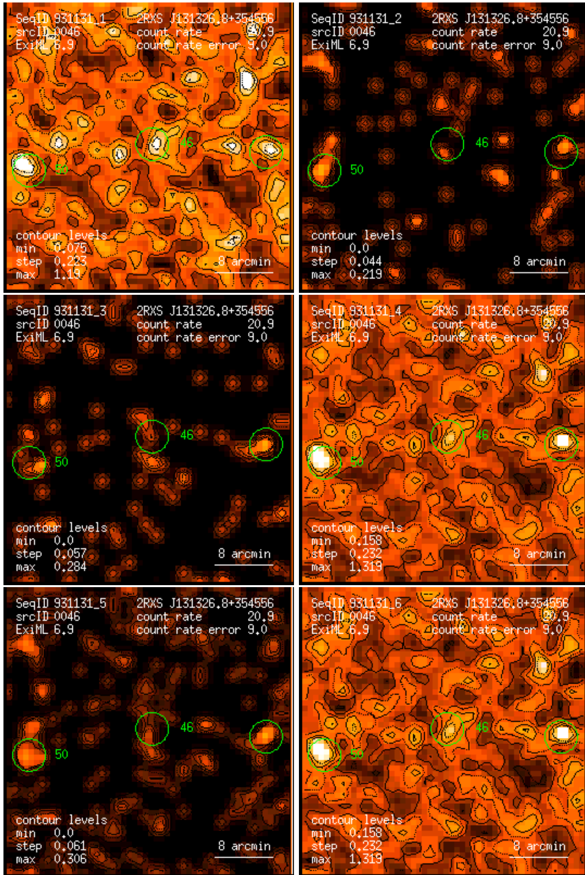
Figure 46: RASS 931131: detection 0046: band rate images, Gaussian filter: (1) PSPC channels 11 – 41, (2) 52 – 90, (3) 91 – 201, (4) 11 – 235, (5) 52 – 201, (6) 11 – 201. Broad band rates in counts/ks. Band rate contour levels in counts/ks/arcmin 2 .
