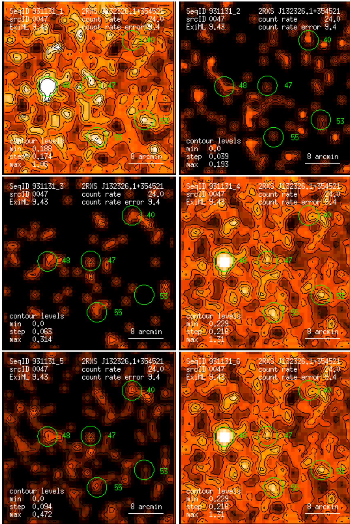
Figure 47: RASS 931131: detection 0047: band rate images, Gaussian filter: (1) PSPC channels 11 – 41, (2) 52 – 90, (3) 91 – 201, (4) 11 – 235, (5) 52 – 201, (6) 11 – 201. Broad band rates in counts/ks. Band rate contour levels in counts/ks/arcmin 2 .
