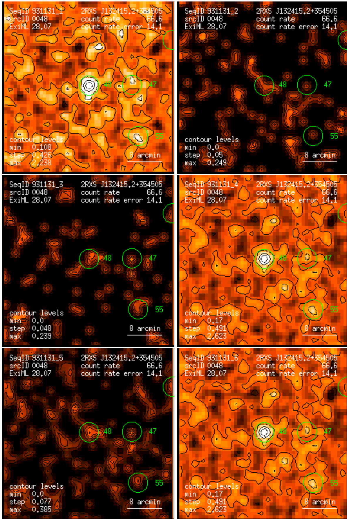
Figure 48: RASS 931131: detection 0048: band rate images, Gaussian filter: (1) PSPC channels 11 – 41, (2) 52 – 90, (3) 91 – 201, (4) 11 – 235, (5) 52 – 201, (6) 11 – 201. Broad band rates in counts/ks. Band rate contour levels in counts/ks/arcmin 2 .
