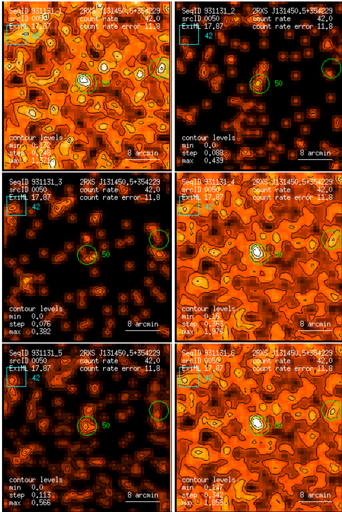
Figure 50: RASS 931131: detection 0050: band rate images, Gaussian filter: (1) PSPC channels 11 – 41, (2) 52 – 90, (3) 91 – 201, (4) 11 – 235, (5) 52 – 201, (6) 11 – 201. Broad band rates in counts/ks. Band rate contour levels in counts/ks/arcmin 2 .
