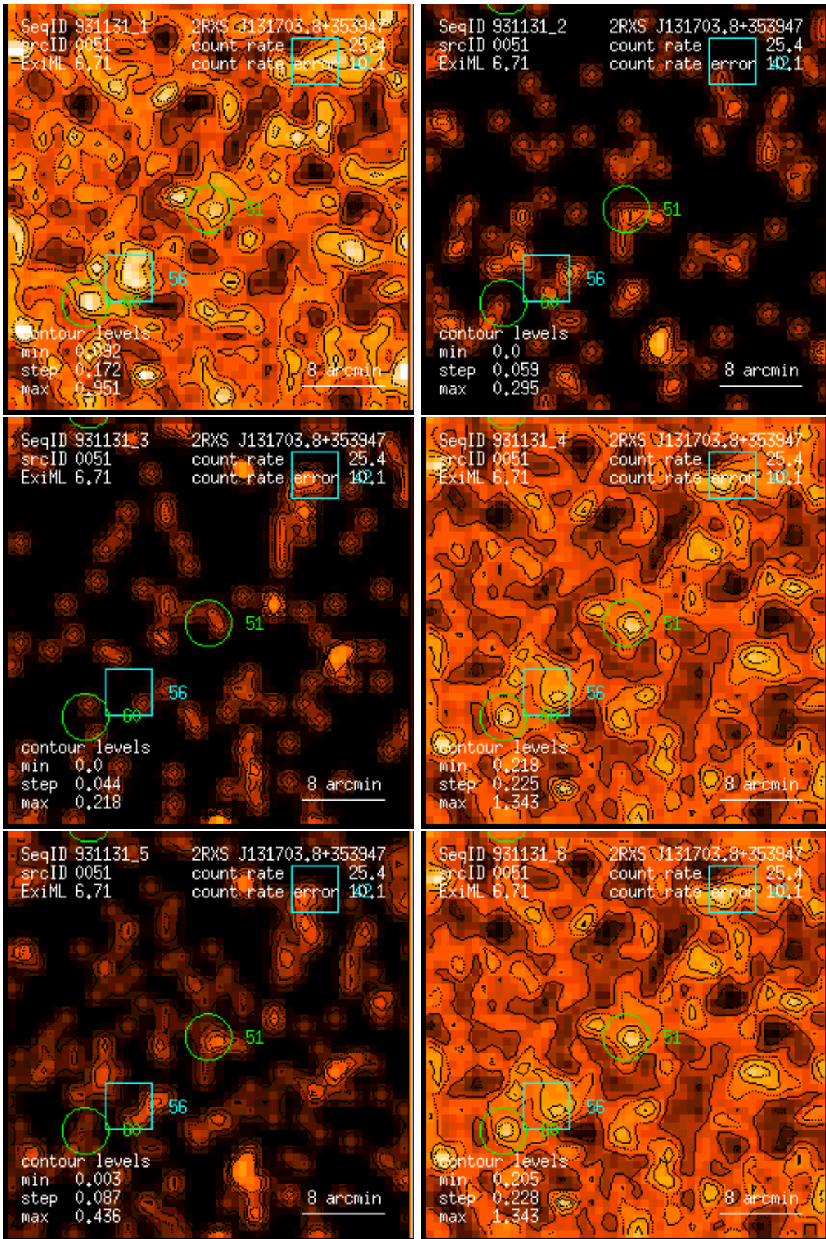
Figure 51: RASS 931131: detection 0051: band rate images, Gaussian filter: (1) PSPC channels 11 – 41, (2) 52 – 90, (3) 91 – 201, (4) 11 – 235, (5) 52 – 201, (6) 11 – 201. Broad band rates in counts/ks. Band rate contour levels in counts/ks/arcmin 2 .
