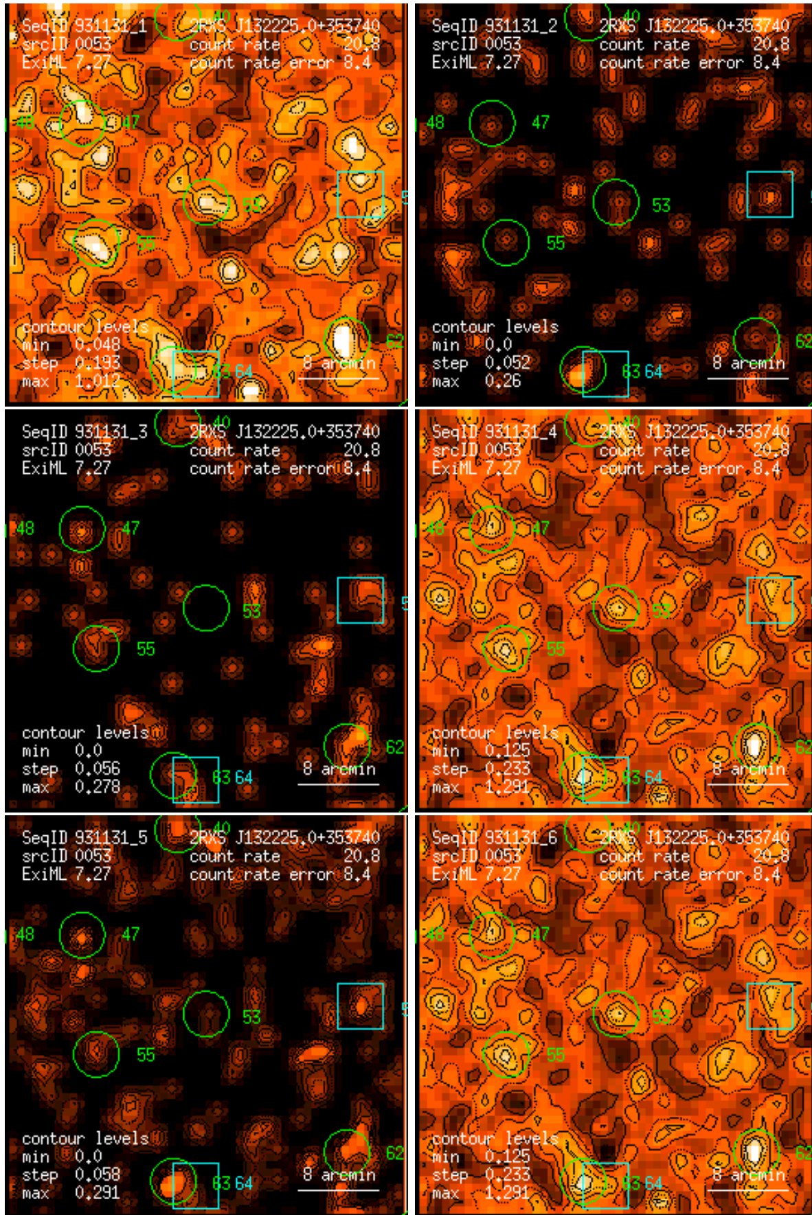
Figure 53: RASS 931131: detection 0053: band rate images, Gaussian filter: (1) PSPC channels 11 – 41, (2) 52 – 90, (3) 91 – 201, (4) 11 – 235, (5) 52 – 201, (6) 11 – 201. Broad band rates in counts/ks. Band rate contour levels in counts/ks/arcmin 2 .
