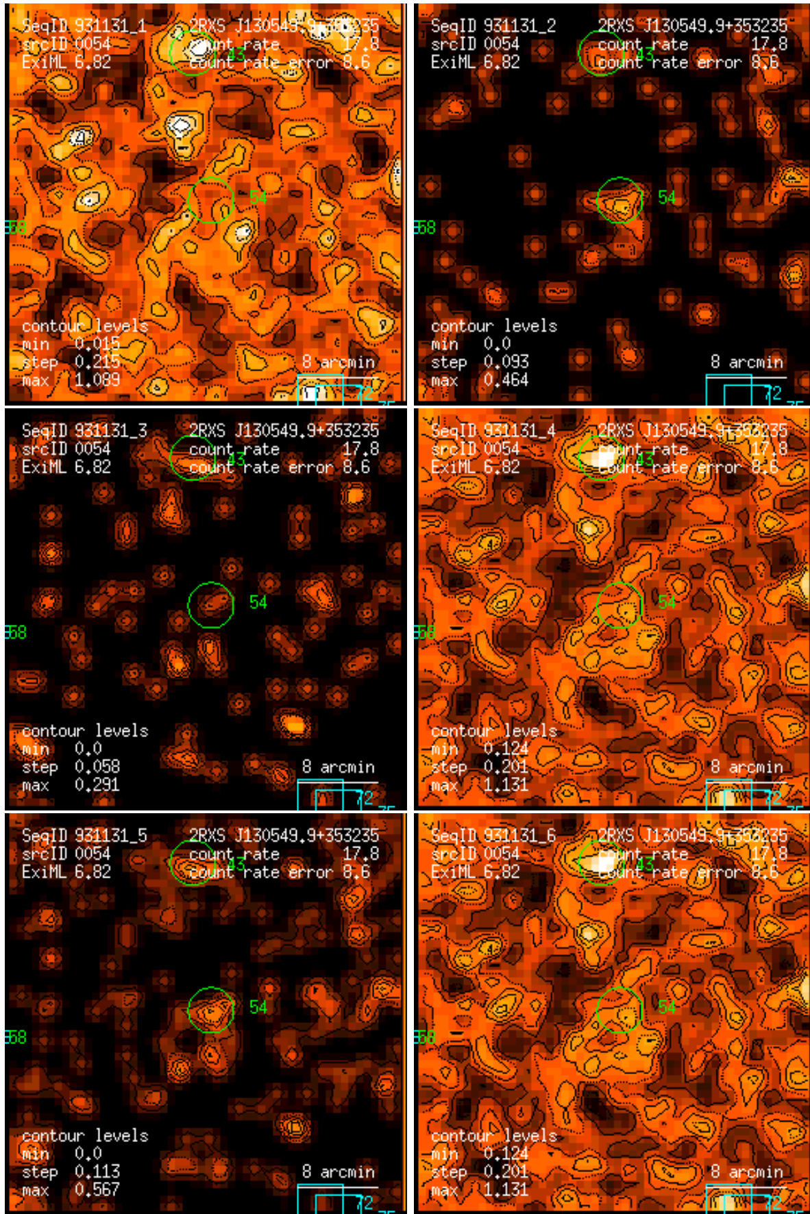
Figure 54: RASS 931131: detection 0054: band rate images, Gaussian filter: (1) PSPC channels 11 – 41, (2) 52 – 90, (3) 91 – 201, (4) 11 – 235, (5) 52 – 201, (6) 11 – 201. Broad band rates in counts/ks. Band rate contour levels in counts/ks/arcmin 2 .
