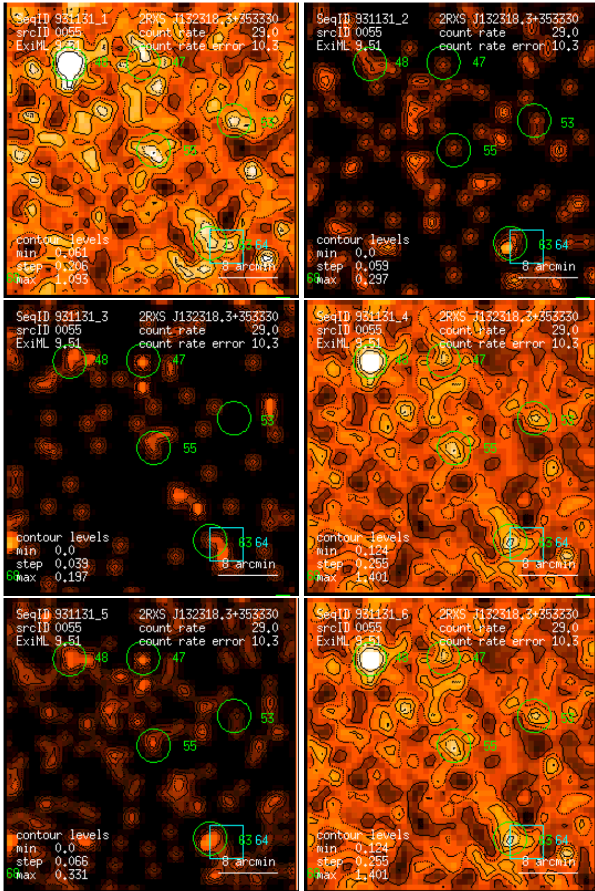
Figure 55: RASS 931131: detection 0055: band rate images, Gaussian filter: (1) PSPC channels 11 – 41, (2) 52 – 90, (3) 91 – 201, (4) 11 – 235, (5) 52 – 201, (6) 11 – 201. Broad band rates in counts/ks. Band rate contour levels in counts/ks/arcmin 2 .
