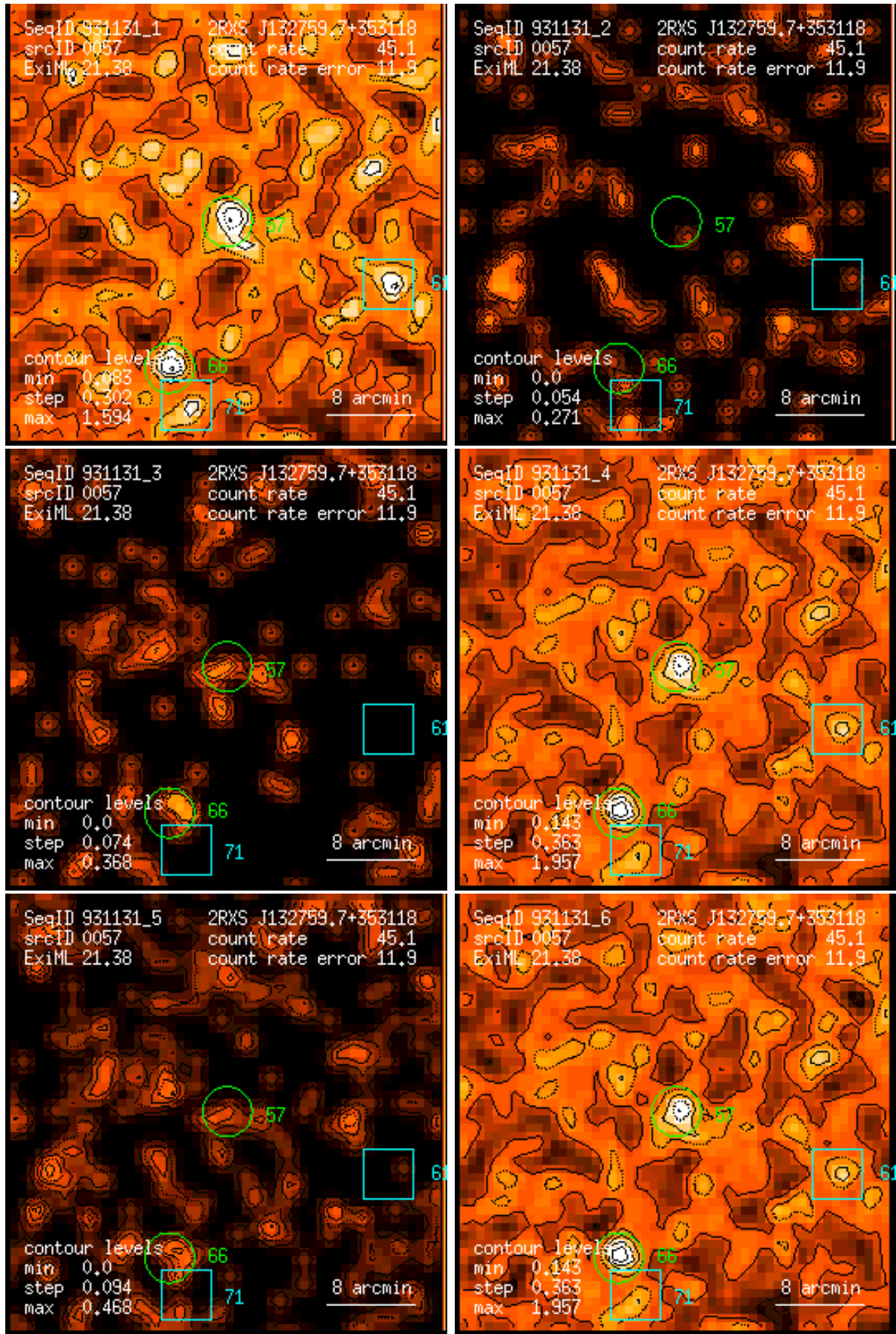
Figure 57: RASS 931131: detection 0057: band rate images, Gaussian filter: (1) PSPC channels 11 – 41, (2) 52 – 90, (3) 91 – 201, (4) 11 – 235, (5) 52 – 201, (6) 11 – 201. Broad band rates in counts/ks. Band rate contour levels in counts/ks/arcmin 2 .
