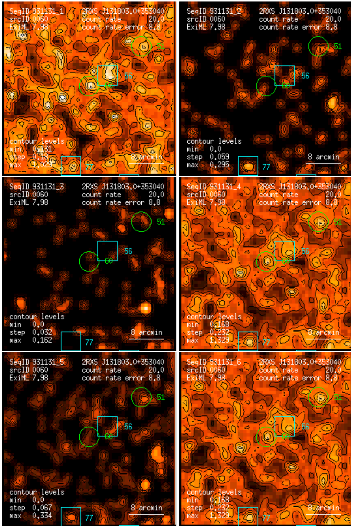
Figure 60: RASS 931131: detection 0060: band rate images, Gaussian filter: (1) PSPC channels 11 – 41, (2) 52 – 90, (3) 91 – 201, (4) 11 – 235, (5) 52 – 201, (6) 11 – 201. Broad band rates in counts/ks. Band rate contour levels in counts/ks/arcmin 2 .
