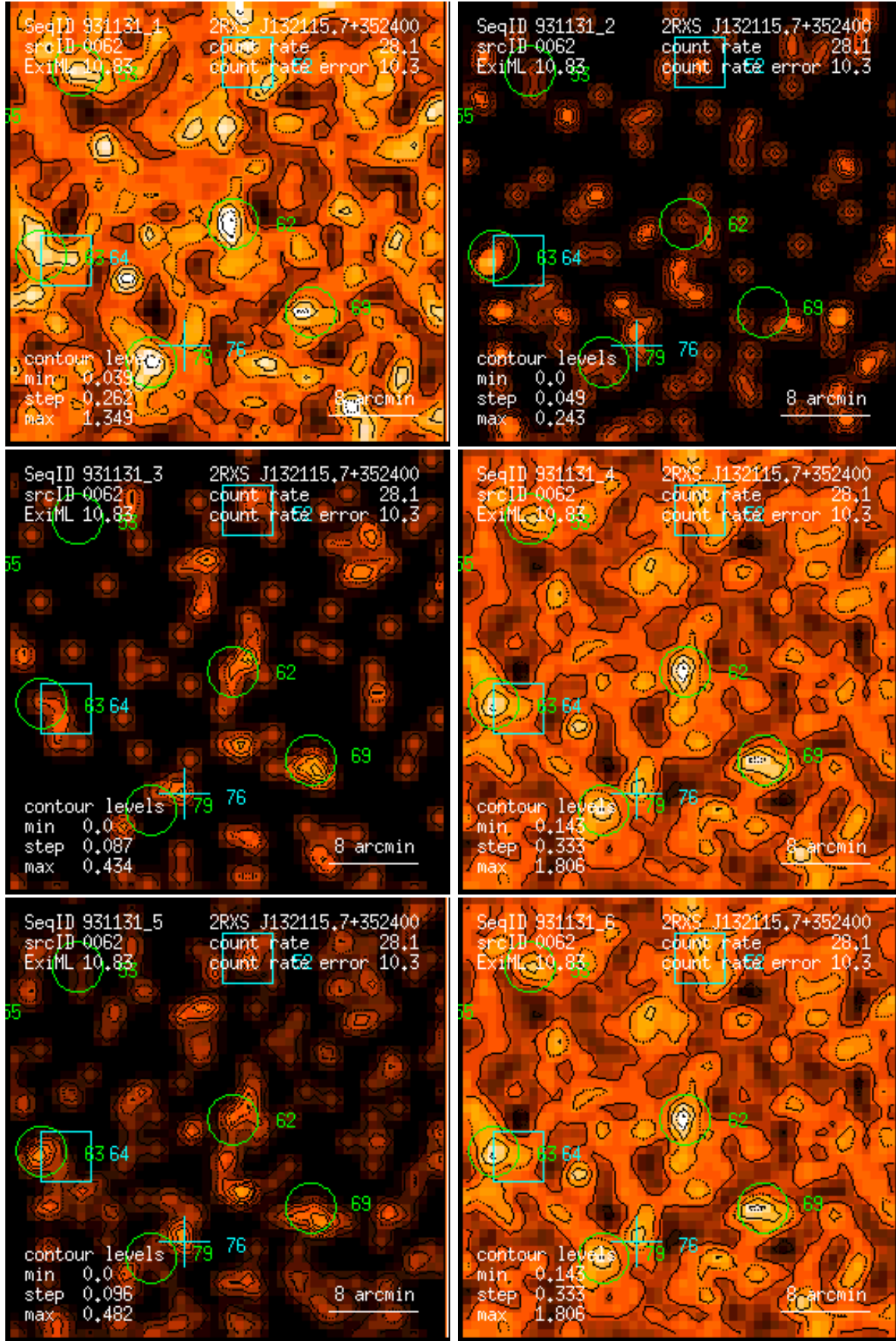
Figure 62: RASS 931131: detection 0062: band rate images, Gaussian filter: (1) PSPC channels 11 – 41, (2) 52 – 90, (3) 91 – 201, (4) 11 – 235, (5) 52 – 201, (6) 11 – 201. Broad band rates in counts/ks. Band rate contour levels in counts/ks/arcmin 2 .
