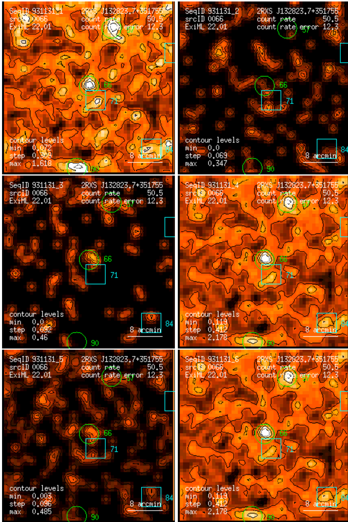
Figure 66: RASS 931131: detection 0066: band rate images, Gaussian filter: (1) PSPC channels 11 – 41, (2) 52 – 90, (3) 91 – 201, (4) 11 – 235, (5) 52 – 201, (6) 11 – 201. Broad band rates in counts/ks. Band rate contour levels in counts/ks/arcmin 2 .
