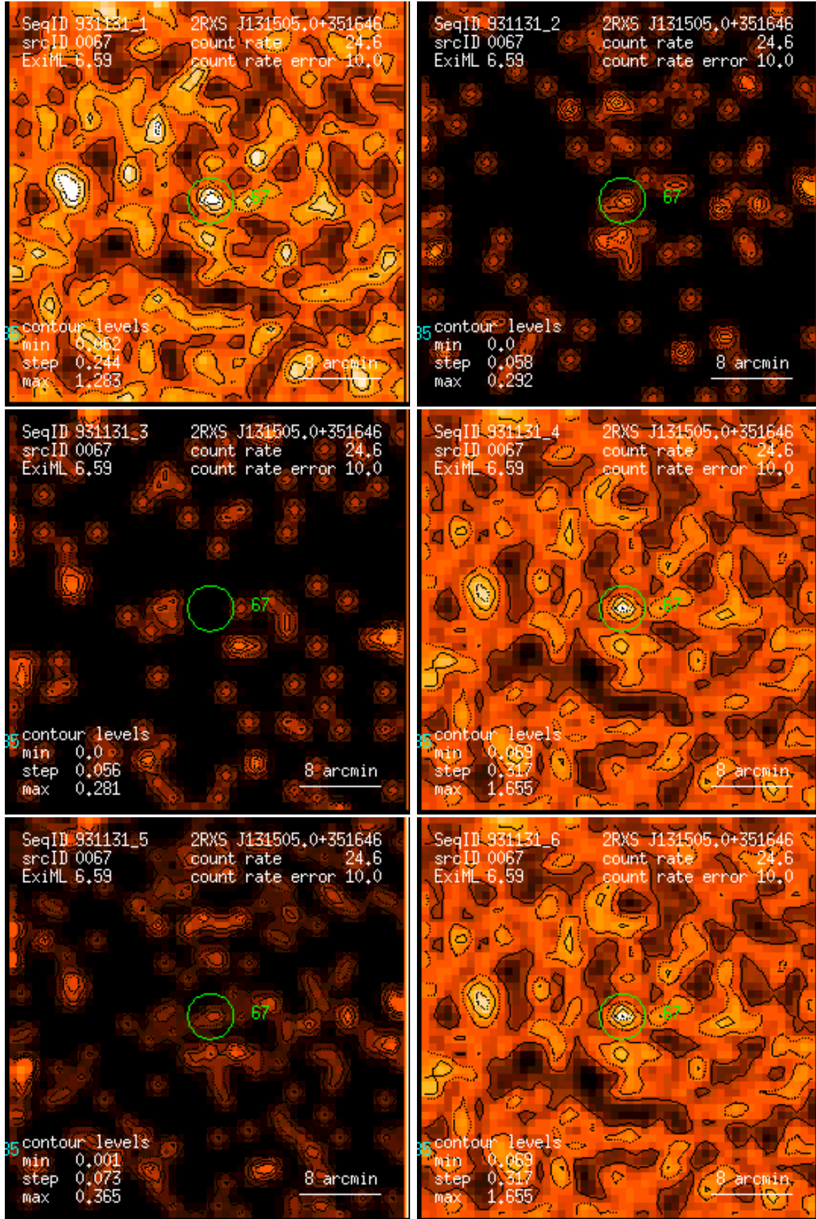
Figure 67: RASS 931131: detection 0067: band rate images, Gaussian filter: (1) PSPC channels 11 – 41, (2) 52 – 90, (3) 91 – 201, (4) 11 – 235, (5) 52 – 201, (6) 11 – 201. Broad band rates in counts/ks. Band rate contour levels in counts/ks/arcmin 2 .
