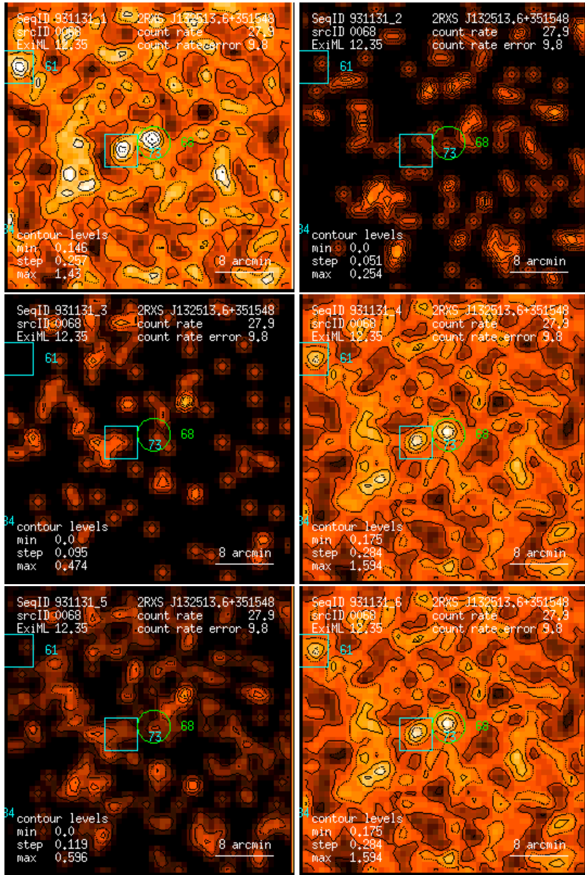
Figure 68: RASS 931131: detection 0068: band rate images, Gaussian filter: (1) PSPC channels 11 – 41, (2) 52 – 90, (3) 91 – 201, (4) 11 – 235, (5) 52 – 201, (6) 11 – 201. Broad band rates in counts/ks. Band rate contour levels in counts/ks/arcmin 2 .
