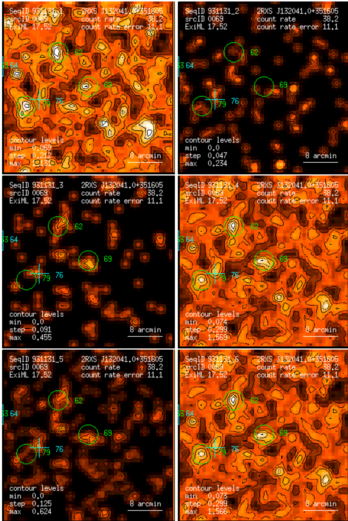
Figure 69: RASS 931131: detection 0069: band rate images, Gaussian filter: (1) PSPC channels 11 – 41, (2) 52 – 90, (3) 91 – 201, (4) 11 – 235, (5) 52 – 201, (6) 11 – 201. Broad band rates in counts/ks. Band rate contour levels in counts/ks/arcmin 2 .
