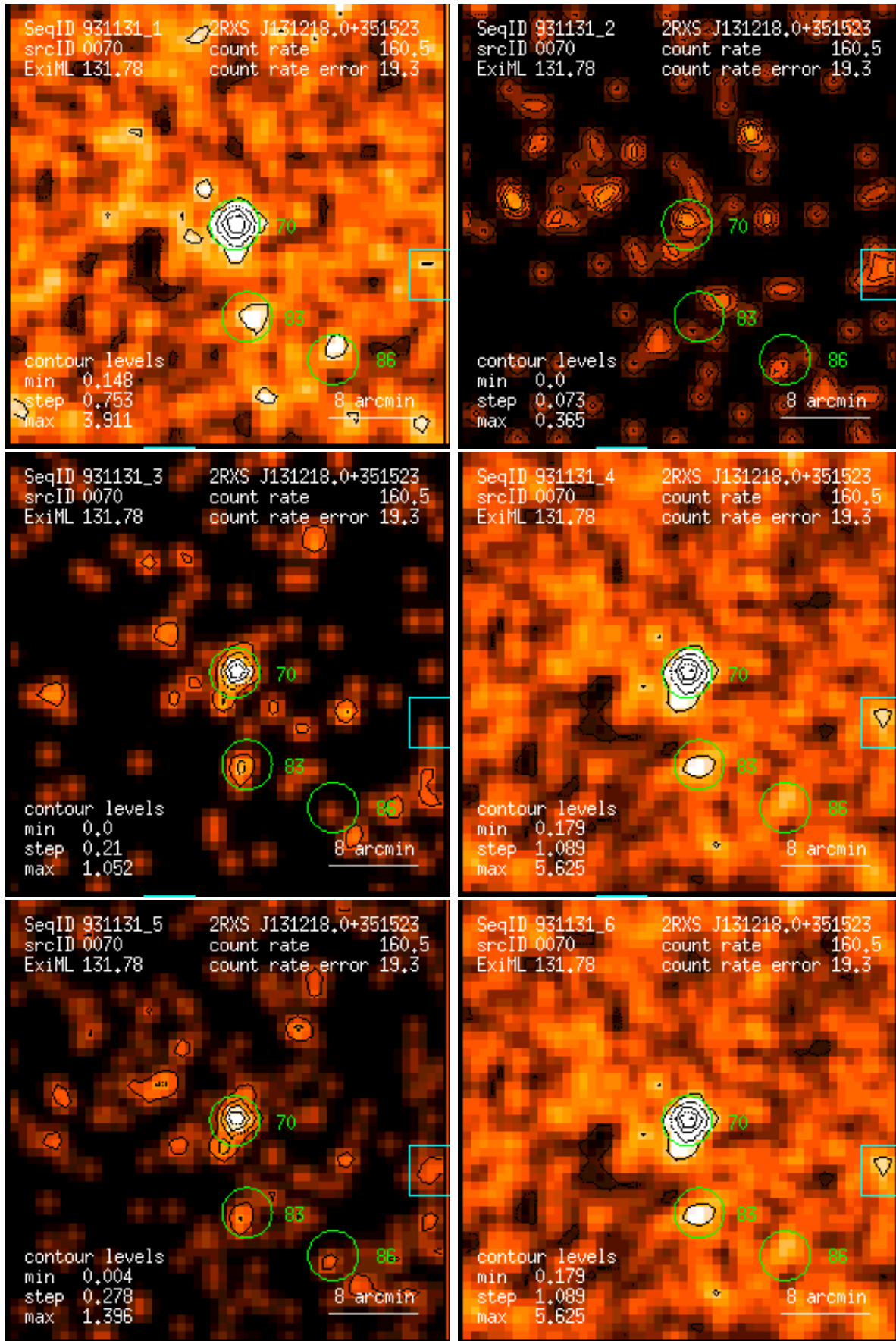
Figure 70: RASS 931131: detection 0070: band rate images, Gaussian filter: (1) PSPC channels 11 – 41, (2) 52 – 90, (3) 91 – 201, (4) 11 – 235, (5) 52 – 201, (6) 11 – 201. Broad band rates in counts/ks. Band rate contour levels in counts/ks/arcmin 2 .
