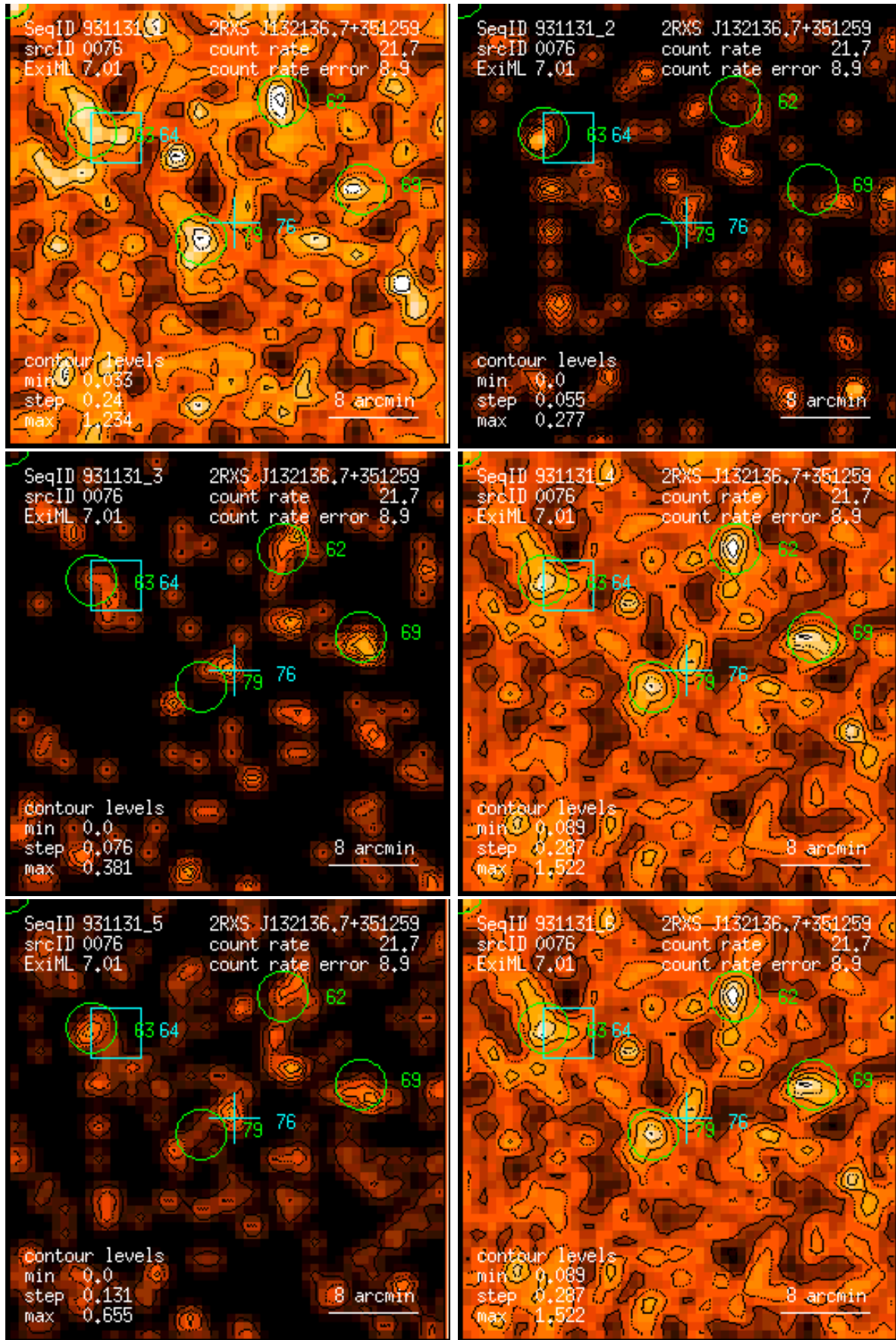
Figure 76: RASS 931131: detection 0076: band rate images, Gaussian filter: (1) PSPC channels 11 – 41, (2) 52 – 90, (3) 91 – 201, (4) 11 – 235, (5) 52 – 201, (6) 11 – 201. Broad band rates in counts/ks. Band rate contour levels in counts/ks/arcmin 2 .
