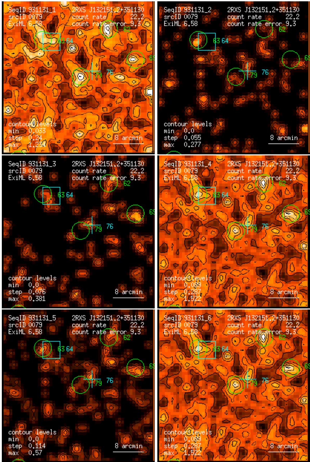
Figure 79: RASS 931131: detection 0079: band rate images, Gaussian filter: (1) PSPC channels 11 – 41, (2) 52 – 90, (3) 91 – 201, (4) 11 – 235, (5) 52 – 201, (6) 11 – 201. Broad band rates in counts/ks. Band rate contour levels in counts/ks/arcmin 2 .
