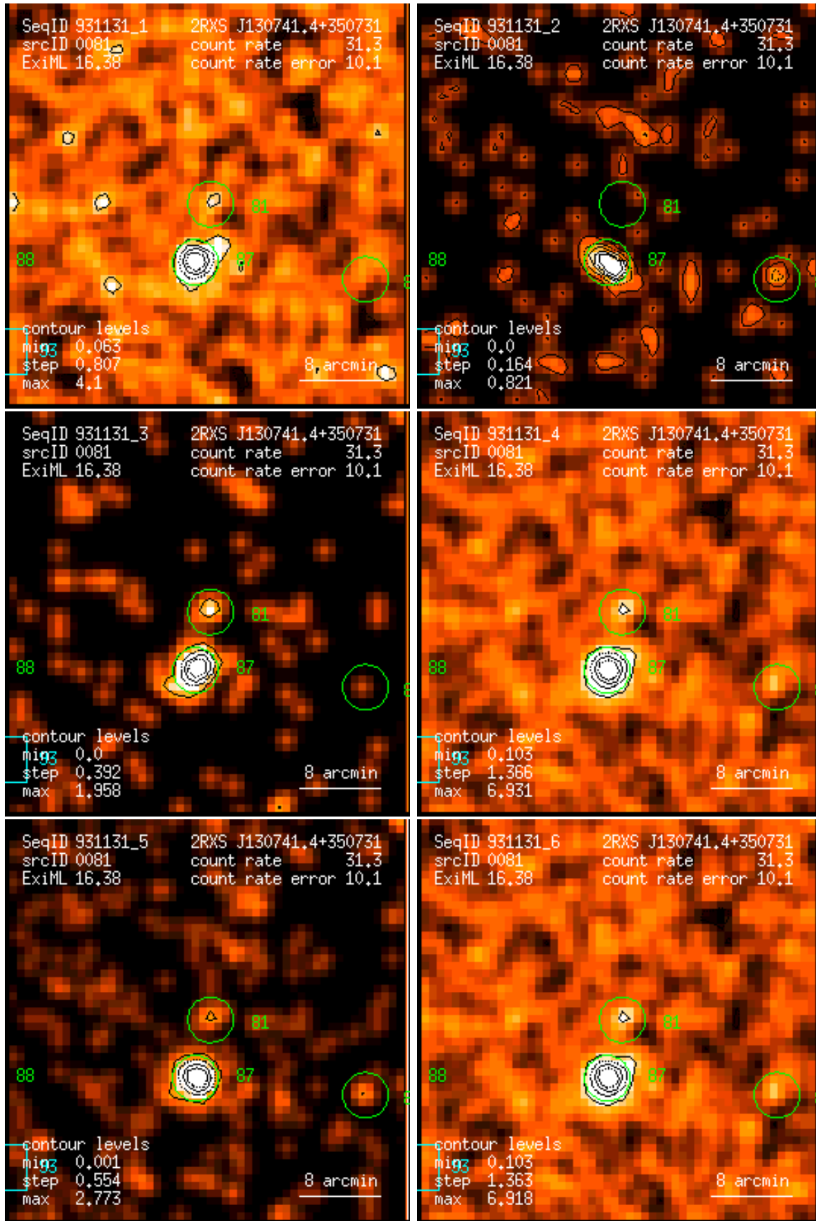
Figure 81: RASS 931131: detection 0081: band rate images, Gaussian filter: (1) PSPC channels 11 – 41, (2) 52 – 90, (3) 91 – 201, (4) 11 – 235, (5) 52 – 201, (6) 11 – 201. Broad band rates in counts/ks. Band rate contour levels in counts/ks/arcmin 2 .
