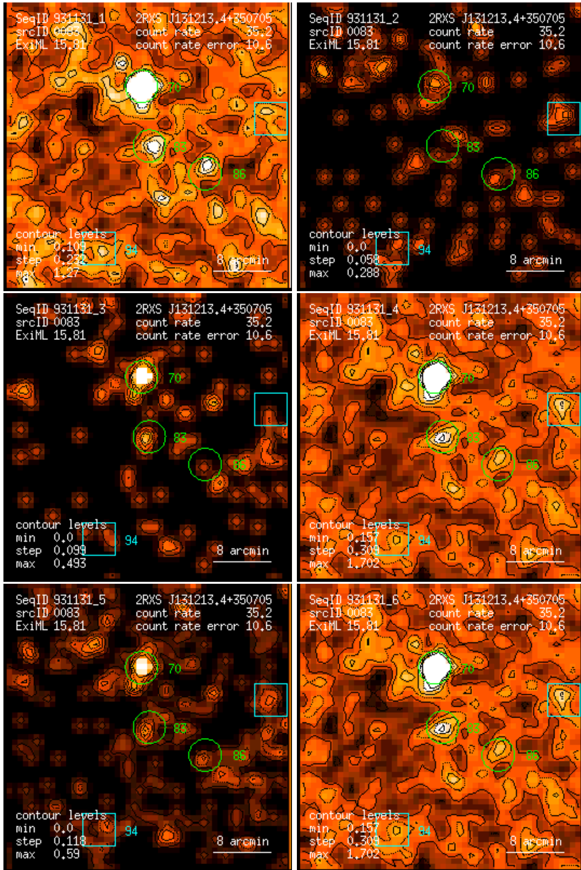
Figure 83: RASS 931131: detection 0083: band rate images, Gaussian filter: (1) PSPC channels 11 – 41, (2) 52 – 90, (3) 91 – 201, (4) 11 – 235, (5) 52 – 201, (6) 11 – 201. Broad band rates in counts/ks. Band rate contour levels in counts/ks/arcmin 2 .
