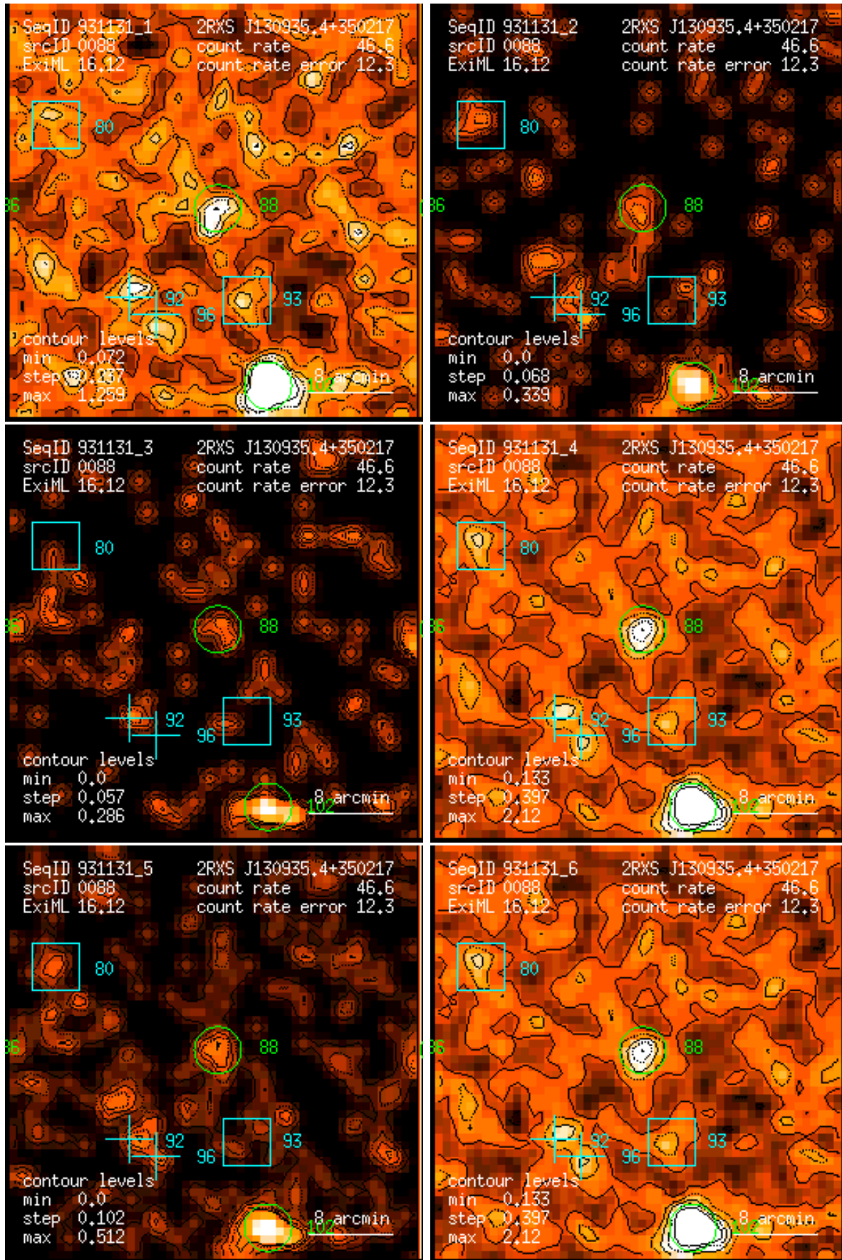
Figure 88: RASS 931131: detection 0088: band rate images, Gaussian filter: (1) PSPC channels 11 – 41, (2) 52 – 90, (3) 91 – 201, (4) 11 – 235, (5) 52 – 201, (6) 11 – 201. Broad band rates in counts/ks. Band rate contour levels in counts/ks/arcmin 2 .
