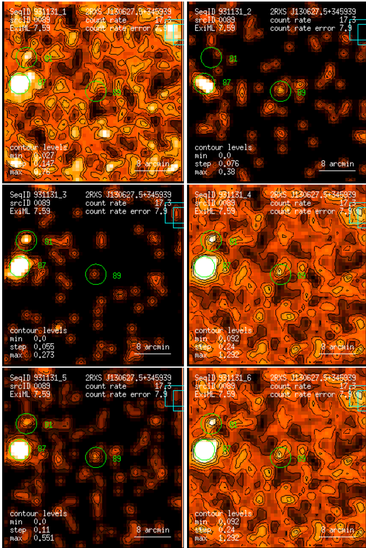
Figure 89: RASS 931131: detection 0089: band rate images, Gaussian filter: (1) PSPC channels 11 – 41, (2) 52 – 90, (3) 91 – 201, (4) 11 – 235, (5) 52 – 201, (6) 11 – 201. Broad band rates in counts/ks. Band rate contour levels in counts/ks/arcmin 2 .
