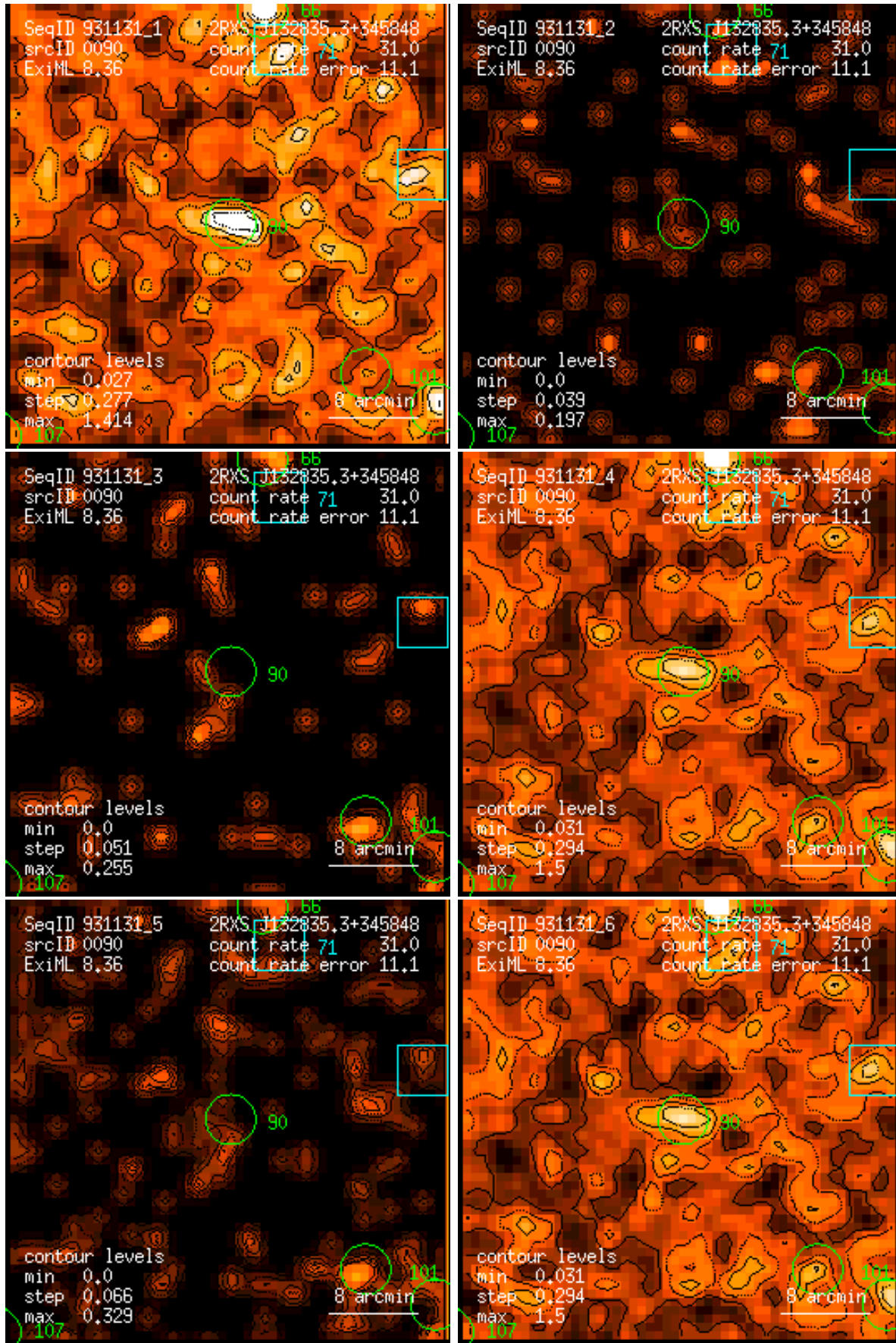
Figure 90: RASS 931131: detection 0090: band rate images, Gaussian filter: (1) PSPC channels 11 – 41, (2) 52 – 90, (3) 91 – 201, (4) 11 – 235, (5) 52 – 201, (6) 11 – 201. Broad band rates in counts/ks. Band rate contour levels in counts/ks/arcmin 2 .
