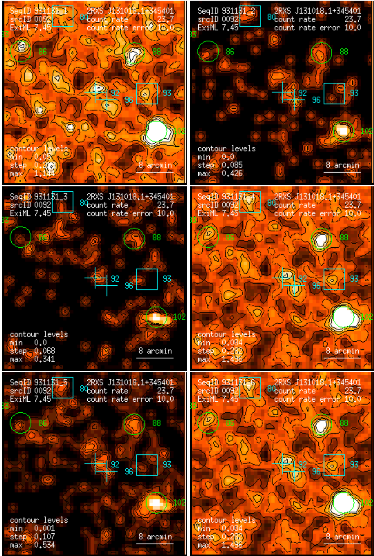
Figure 92: RASS 931131: detection 0092: band rate images, Gaussian filter: (1) PSPC channels 11 – 41, (2) 52 – 90, (3) 91 – 201, (4) 11 – 235, (5) 52 – 201, (6) 11 – 201. Broad band rates in counts/ks. Band rate contour levels in counts/ks/arcmin 2 .
