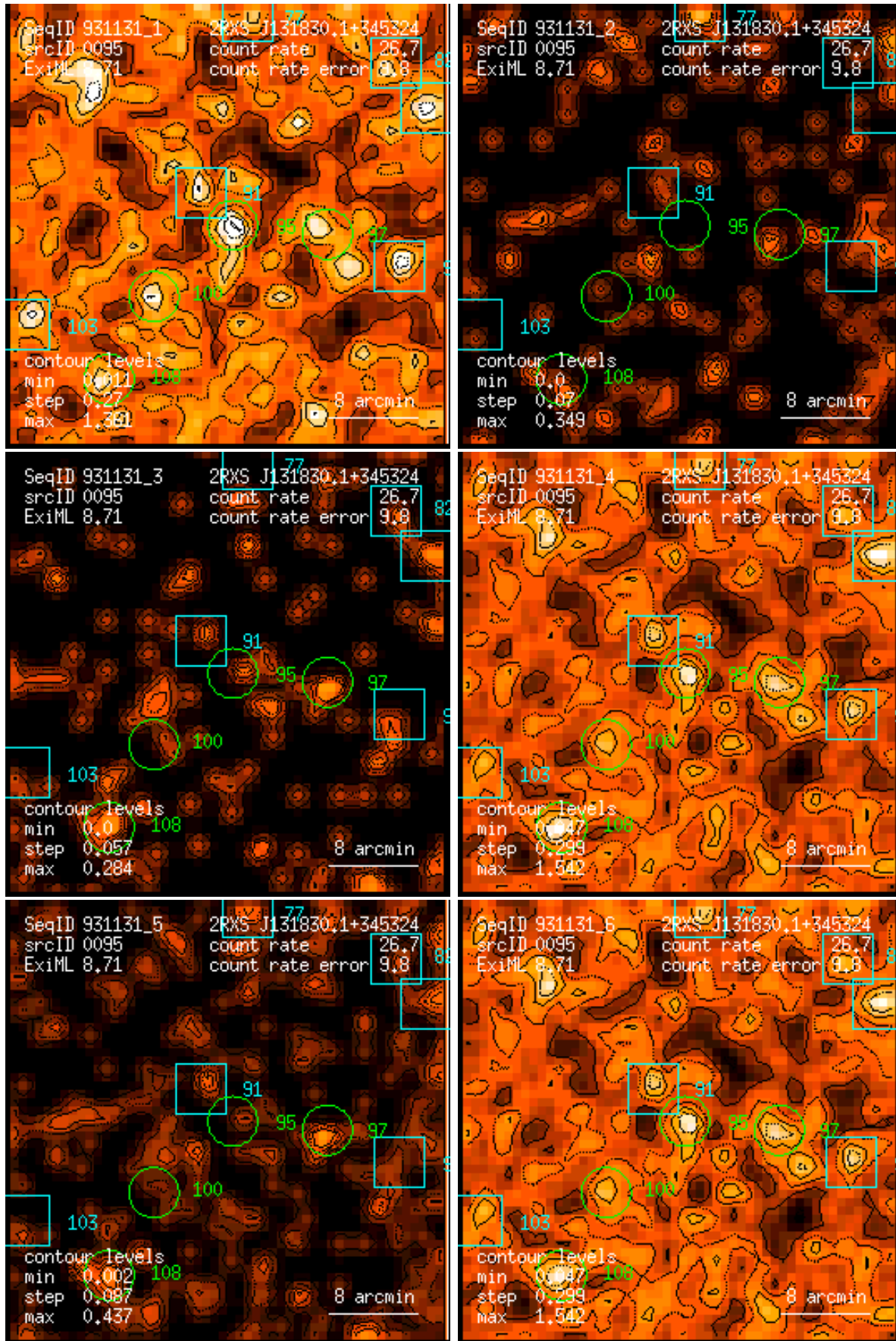
Figure 95: RASS 931131: detection 0095: band rate images, Gaussian filter: (1) PSPC channels 11 – 41, (2) 52 – 90, (3) 91 – 201, (4) 11 – 235, (5) 52 – 201, (6) 11 – 201. Broad band rates in counts/ks. Band rate contour levels in counts/ks/arcmin 2 .
