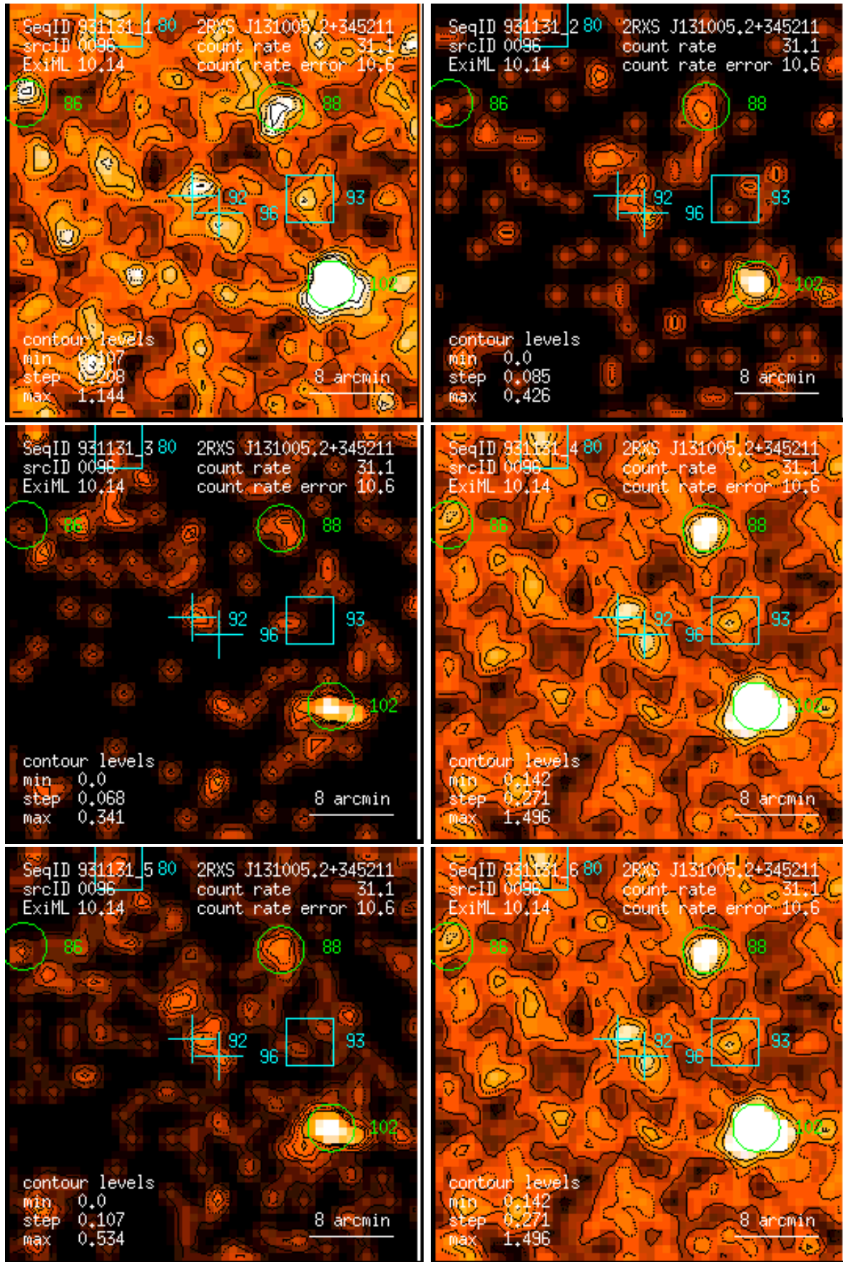
Figure 96: RASS 931131: detection 0096: band rate images, Gaussian filter: (1) PSPC channels 11 – 41, (2) 52 – 90, (3) 91 – 201, (4) 11 – 235, (5) 52 – 201, (6) 11 – 201. Broad band rates in counts/ks. Band rate contour levels in counts/ks/arcmin 2 .
