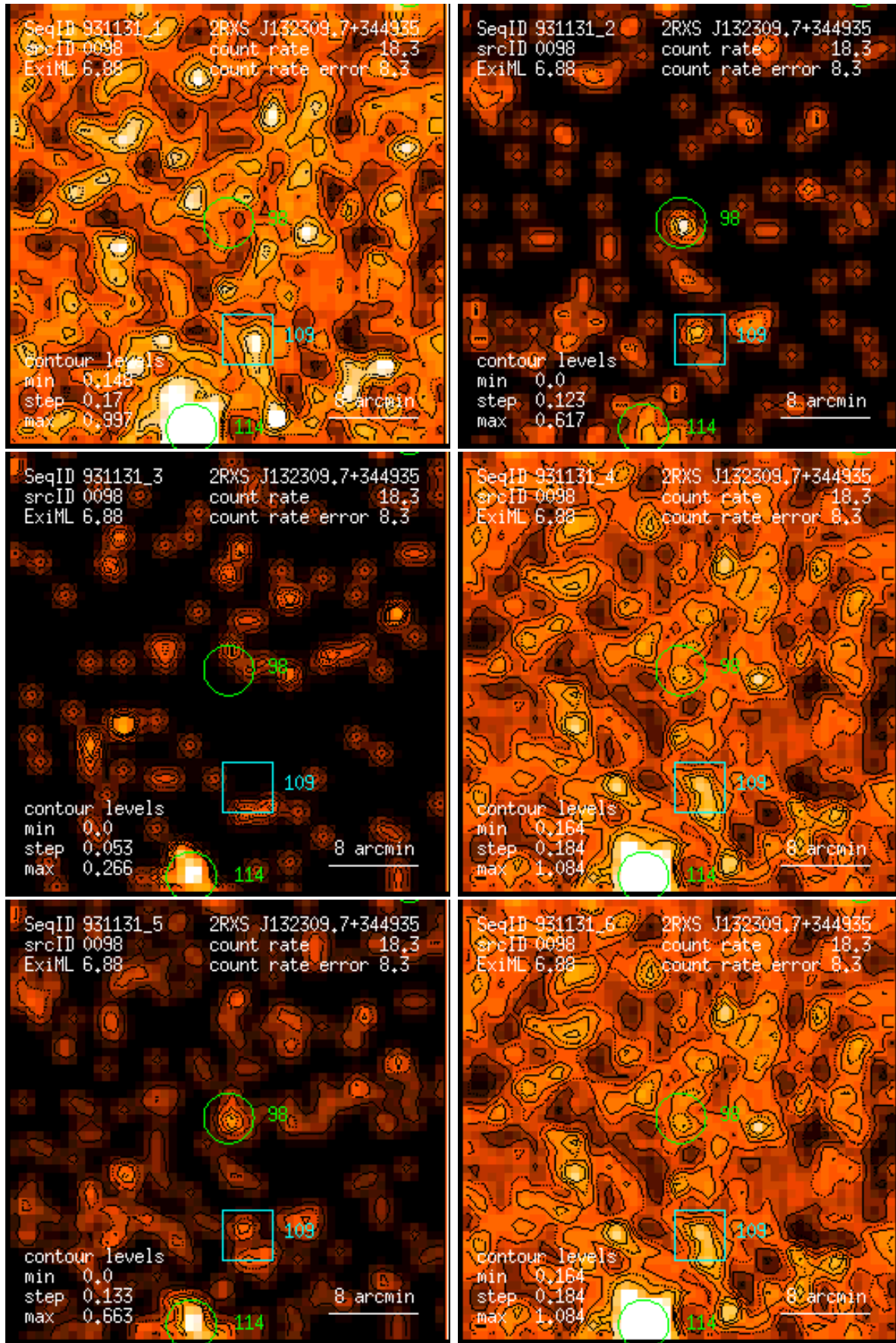
Figure 98: RASS 931131: detection 0098: band rate images, Gaussian filter: (1) PSPC channels 11 – 41, (2) 52 – 90, (3) 91 – 201, (4) 11 – 235, (5) 52 – 201, (6) 11 – 201. Broad band rates in counts/ks. Band rate contour levels in counts/ks/arcmin 2 .
